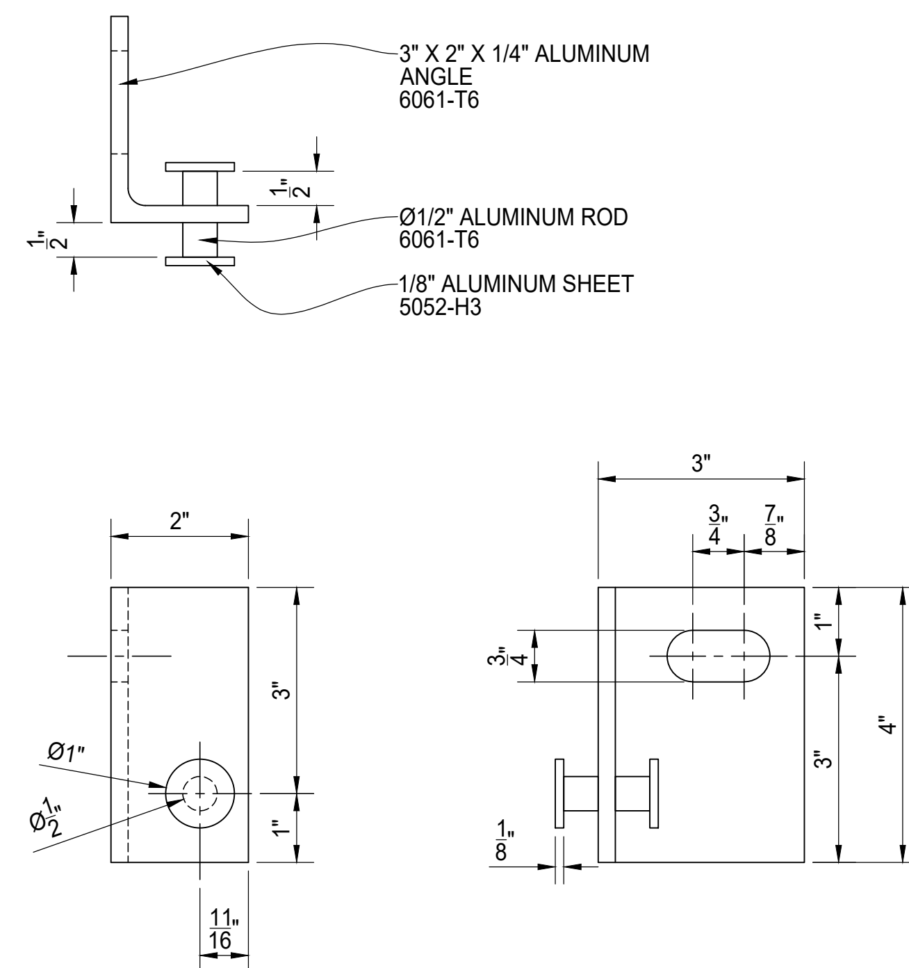
TOP PANEL WALL MOUNT ANGLE CLIP
