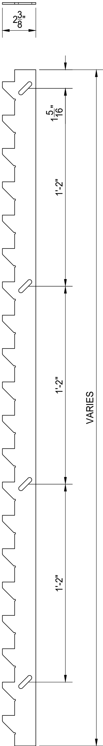
MID-SPAN LOUVER RETAINER BAR 1/8" ALUMINUM LASER CUT FLAT 6061-T6
