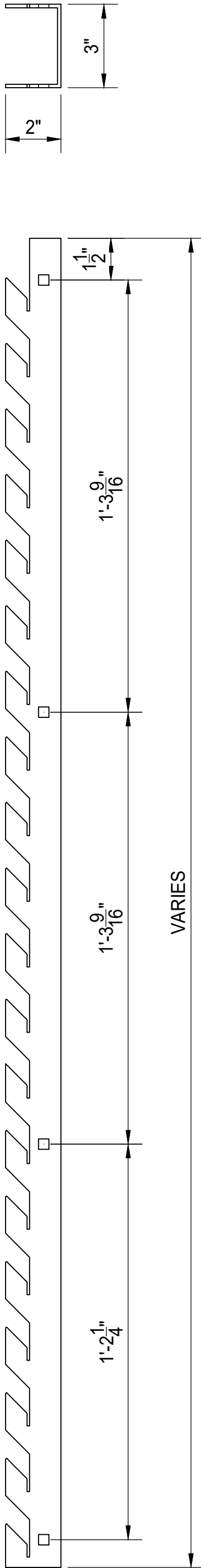
LOUVER SUPPORT CHANNEL 2" X 3" X 1/8" ALUMINUM CHANNEL 6061-T6
