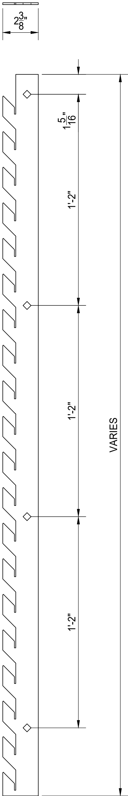
MID-SPAN LOUVER SUPPORT BAR 1/8" ALUMINUM LASER CUT FLAT 6061-T6
