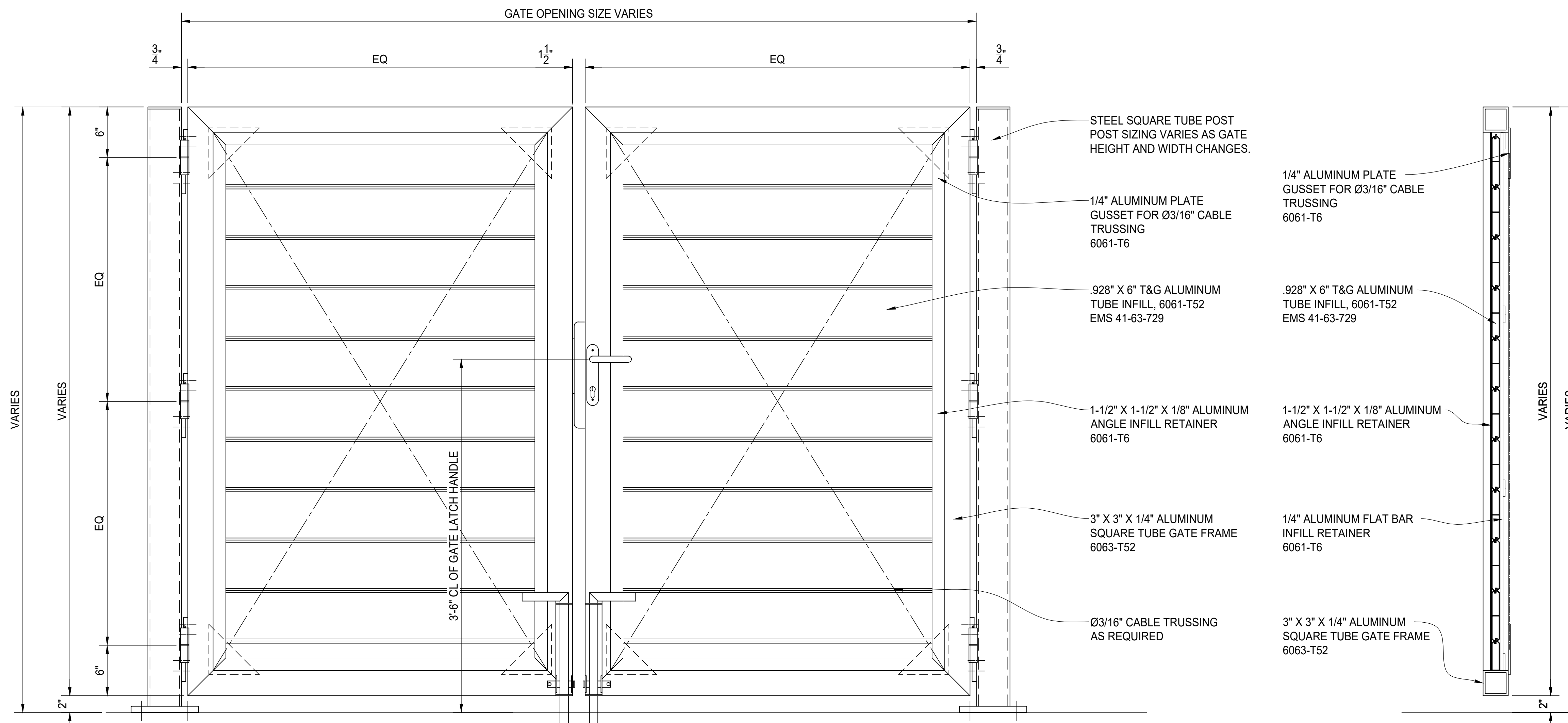
GATE ELEVATION
