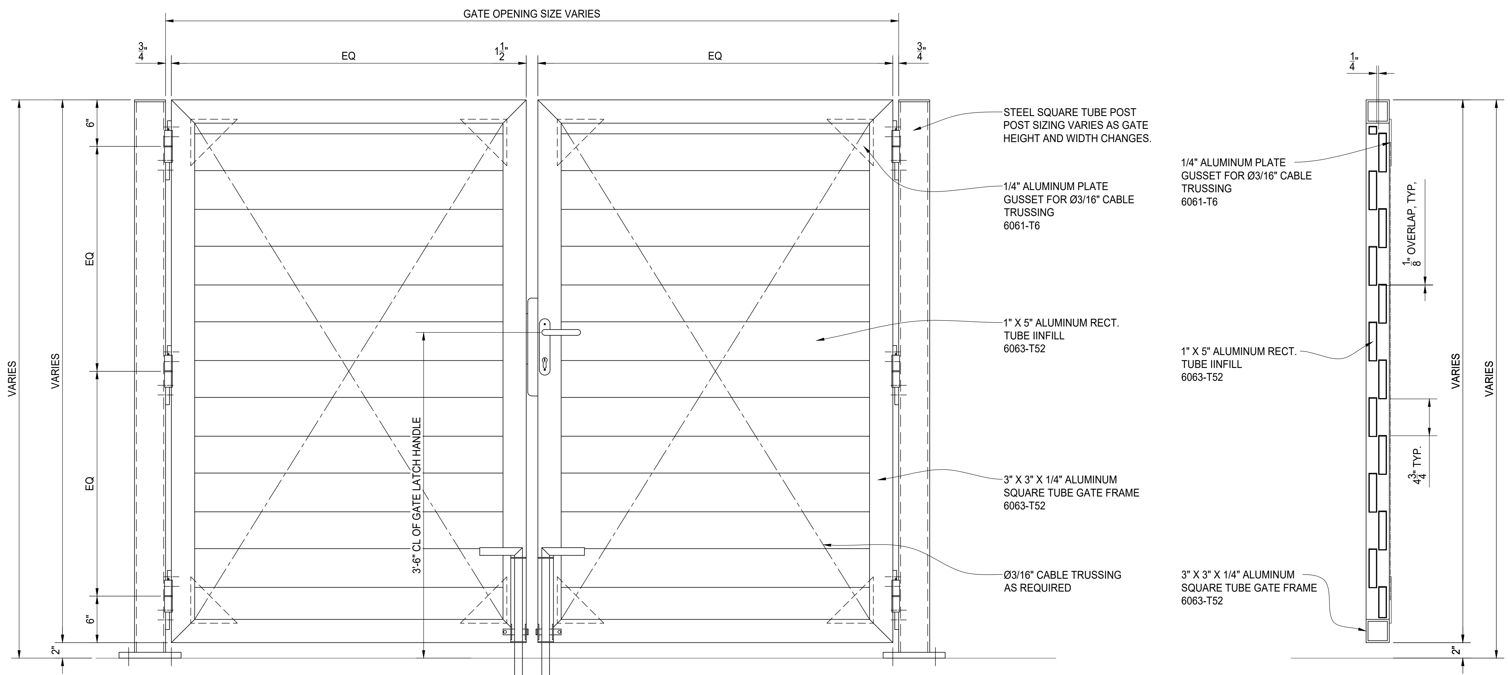
GATE ELEVATION
