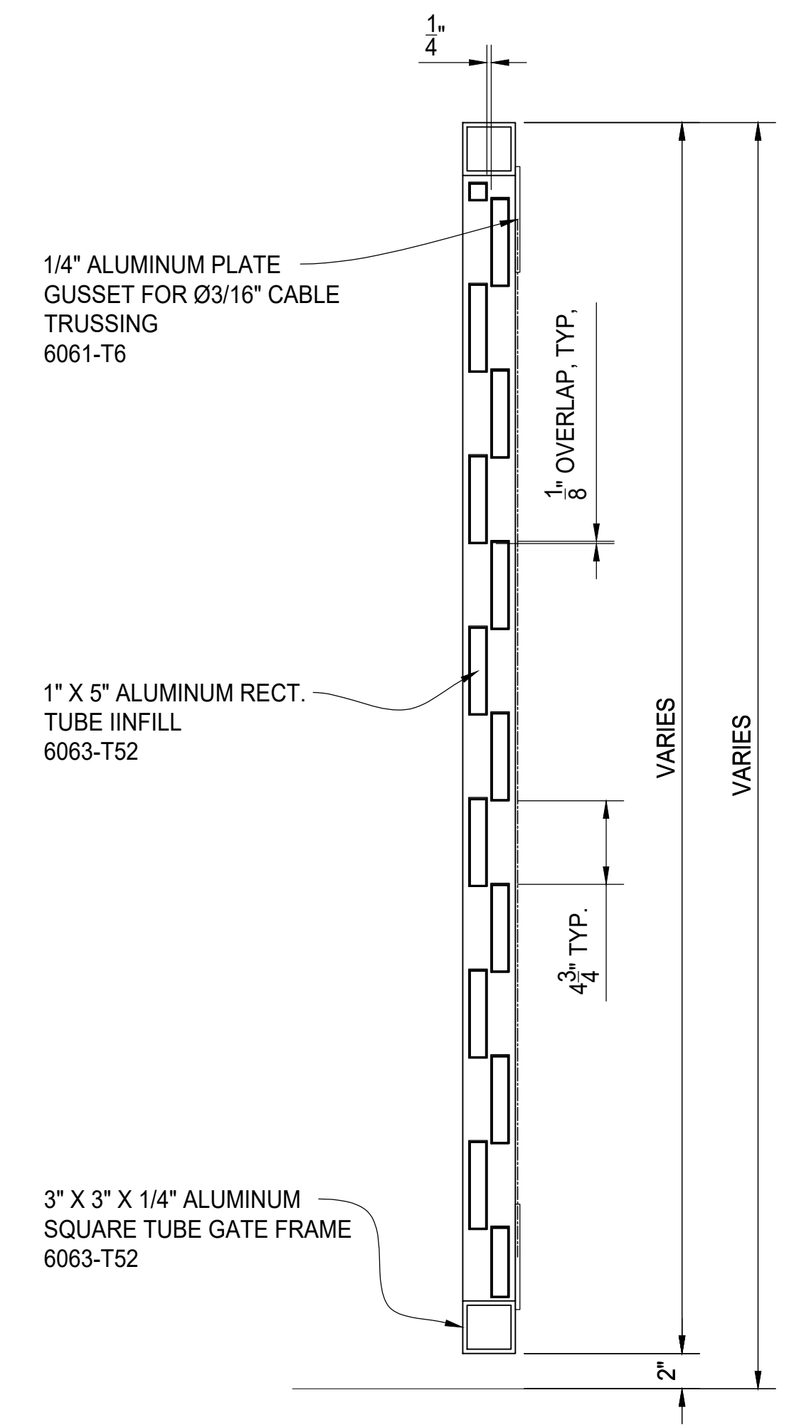
TYPICAL GATE SECTION
