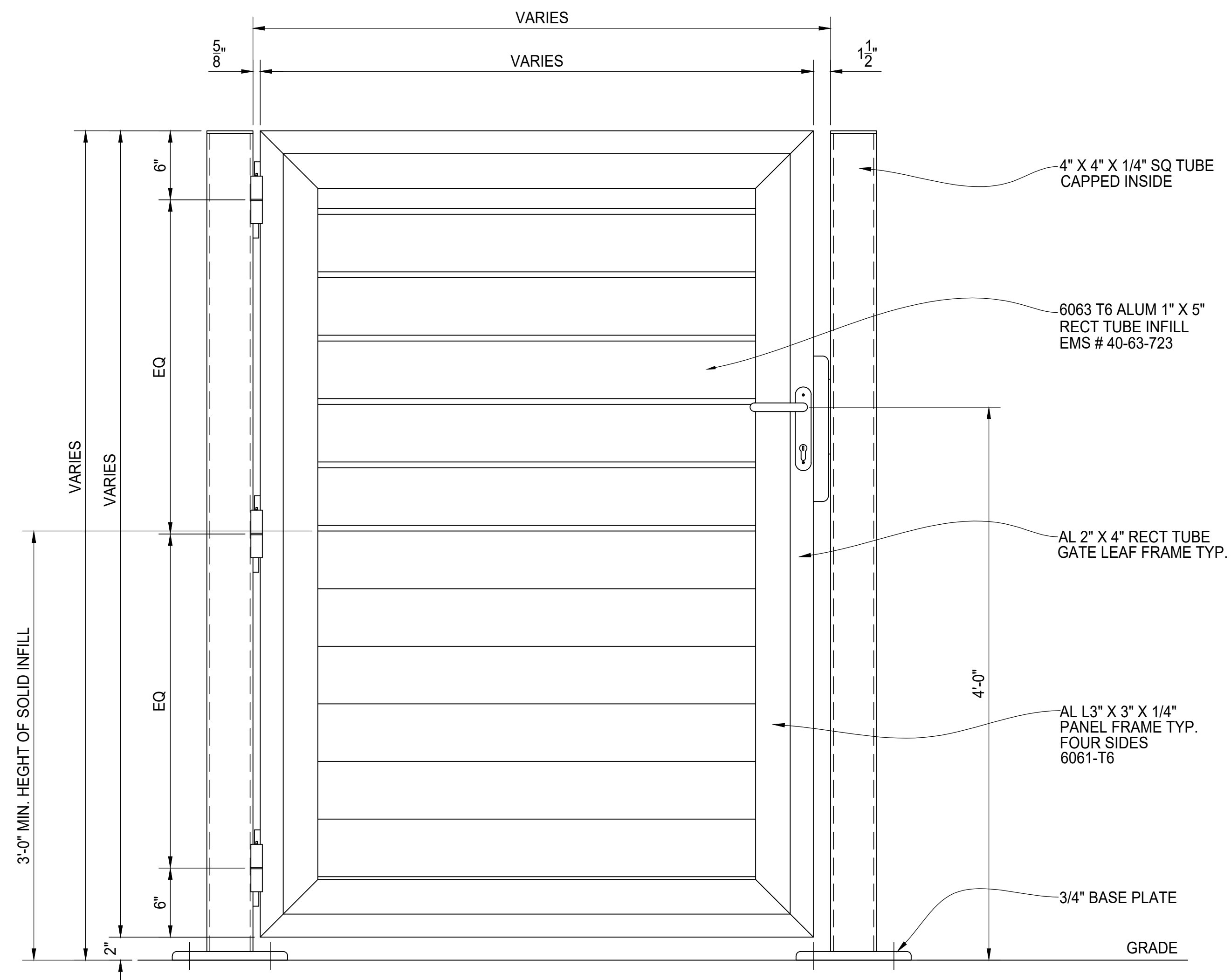
ELEVATION VIEW
