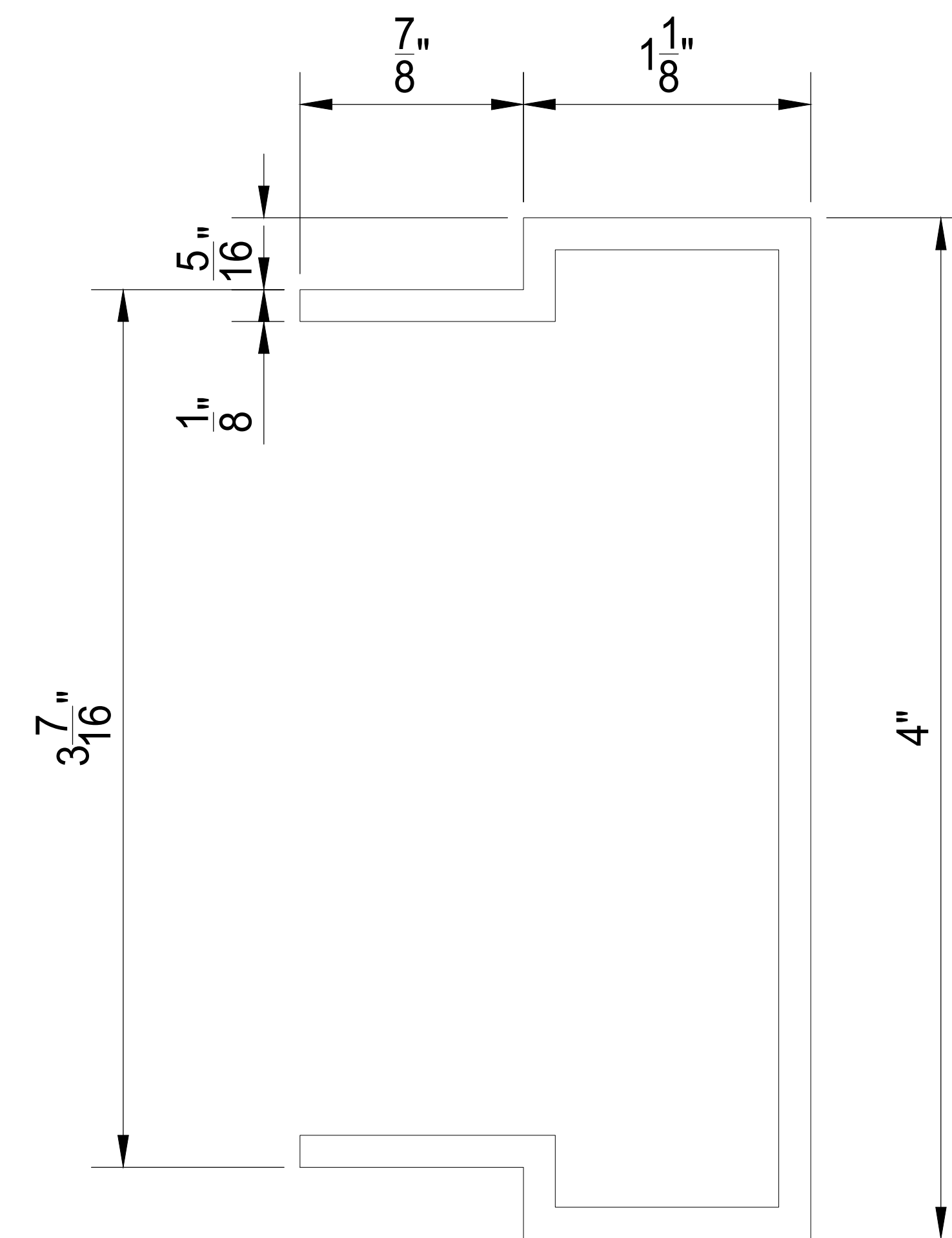
VERTICAL CHANNEL FRAME
