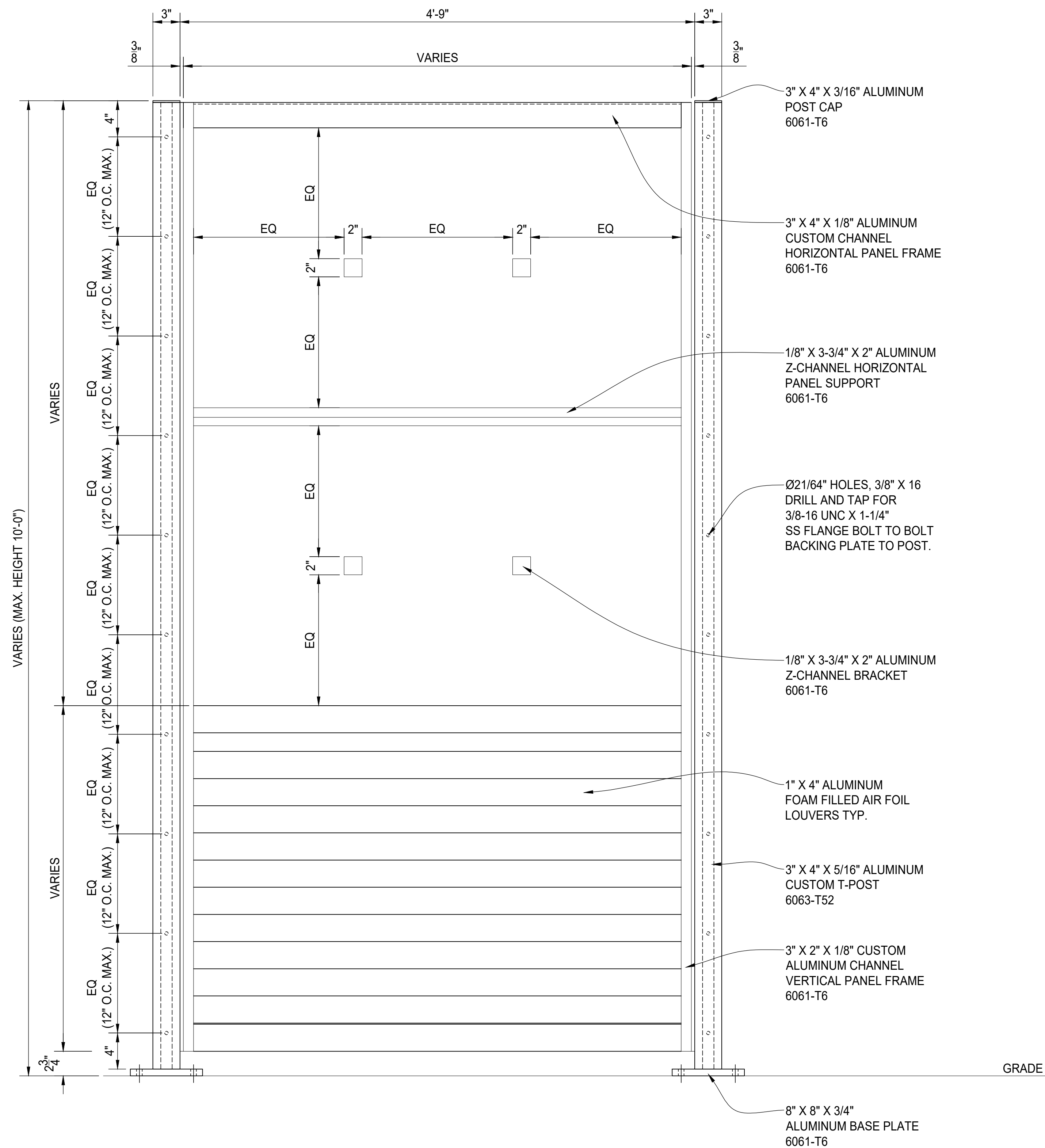
PANEL ELEVATION
