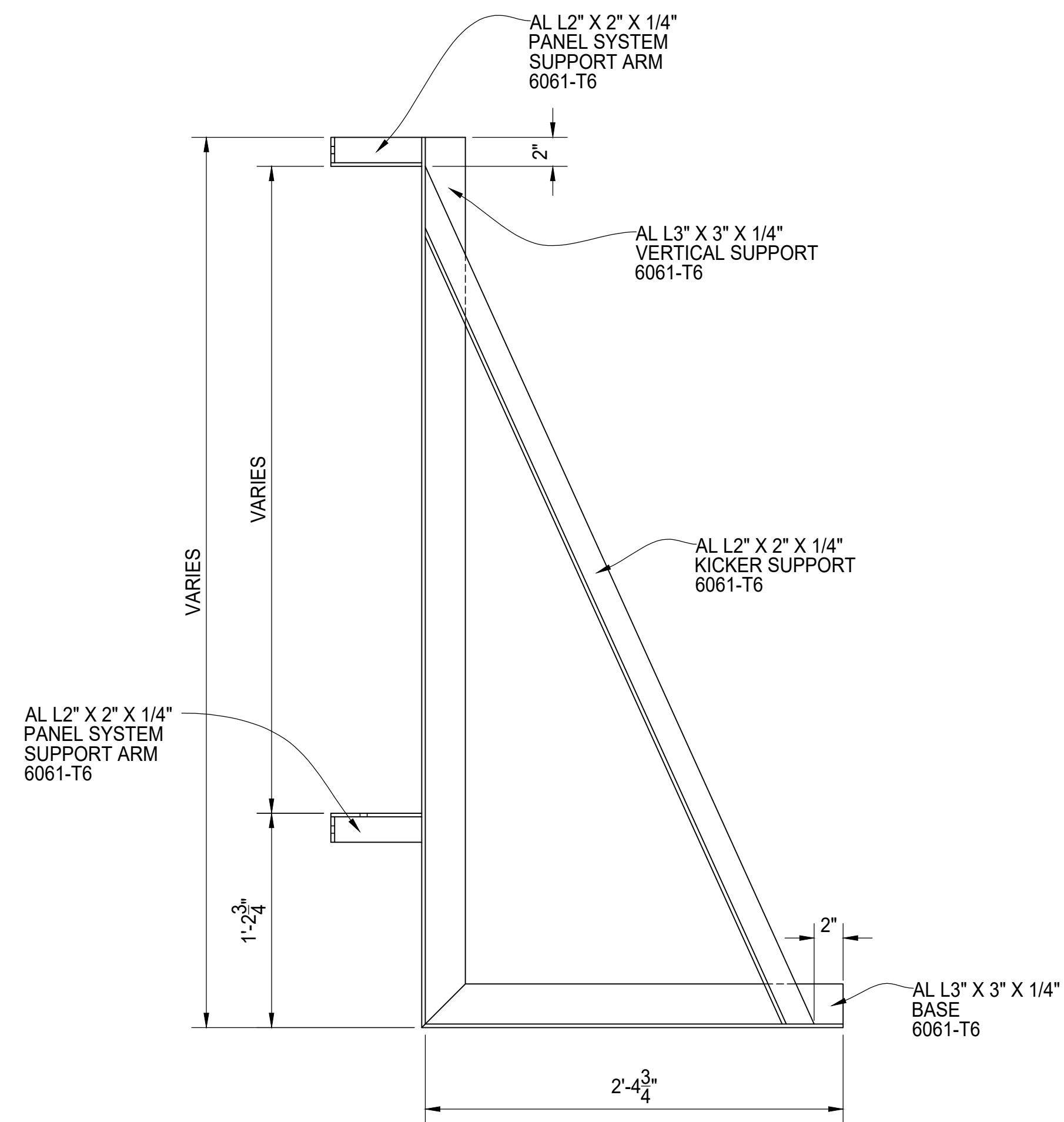
EQUIPMENT MOUNTING BRACKET FOR MOUNTING TO ROOFTOP
