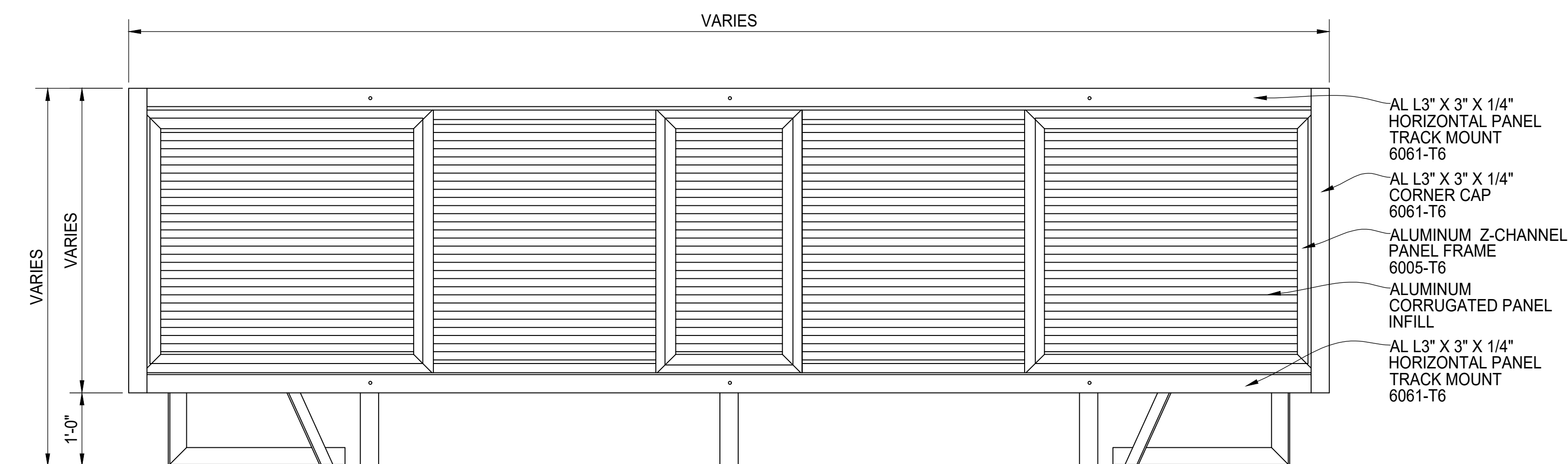
A ELEVATION VIEW QUANTITY OF PANELS AND MOUNTING BRACKETS WILL BE DEPENDANT ON THE ROOFTOP EQUIPMENT SIZE.
