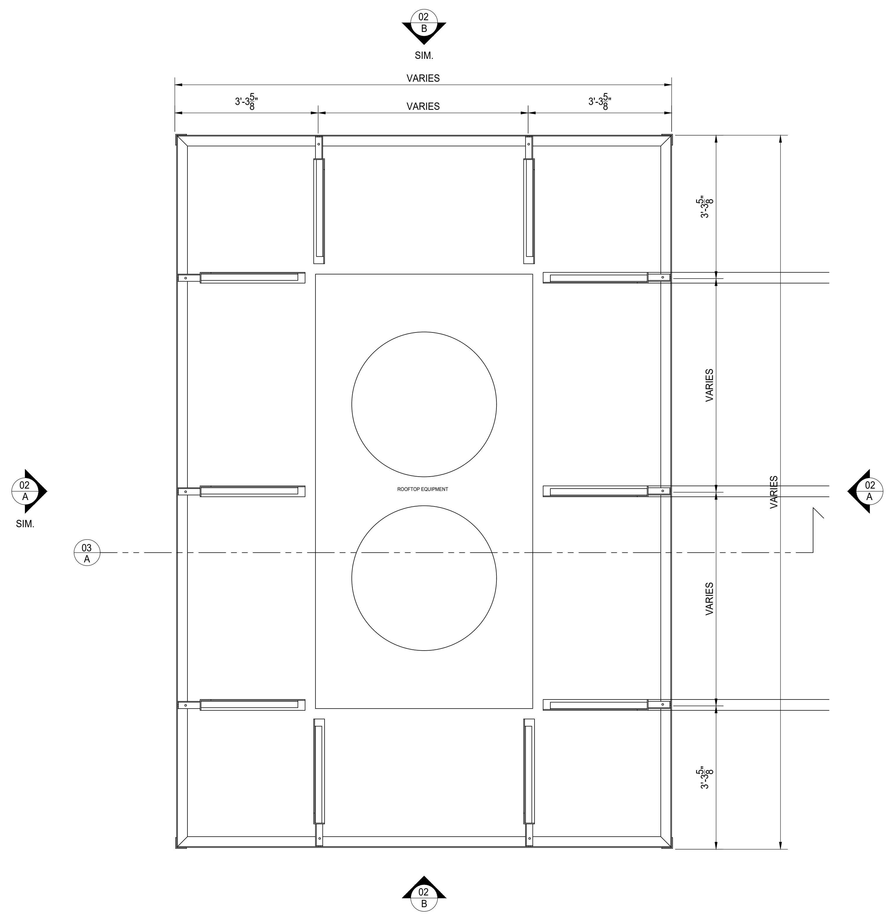
PLAN VIEW
