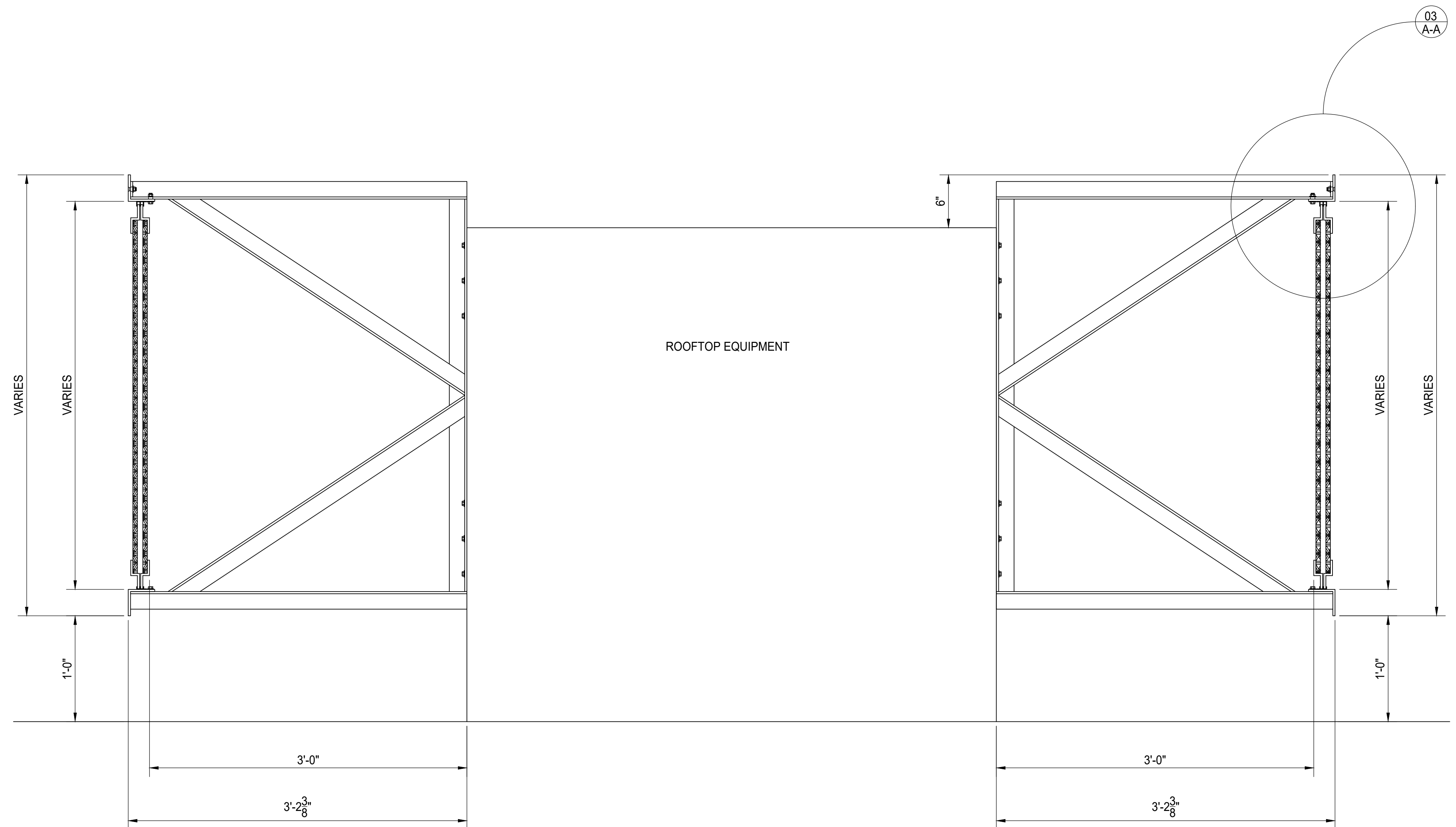
A SECTION VIEW OF ROOFTOP SCREENING
