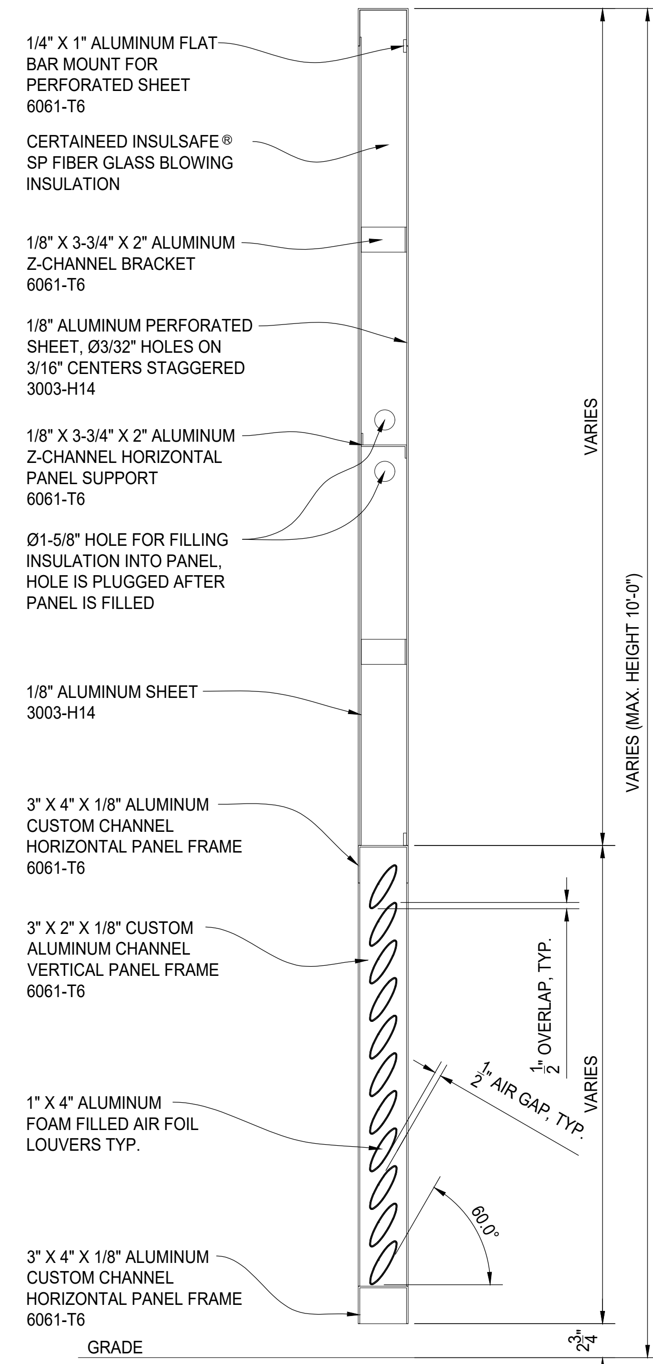
TYPICAL PANEL SECTION
