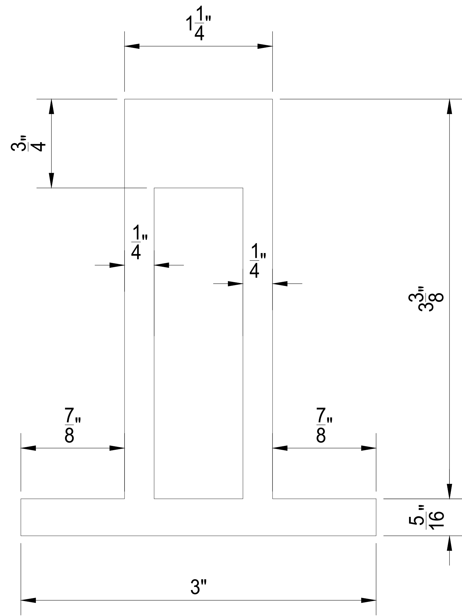
CUSTOM POST
