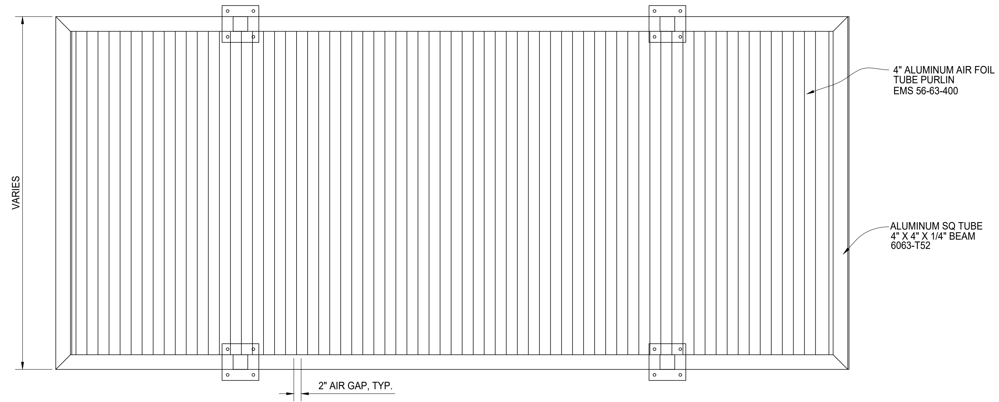
PLAN VIEW
