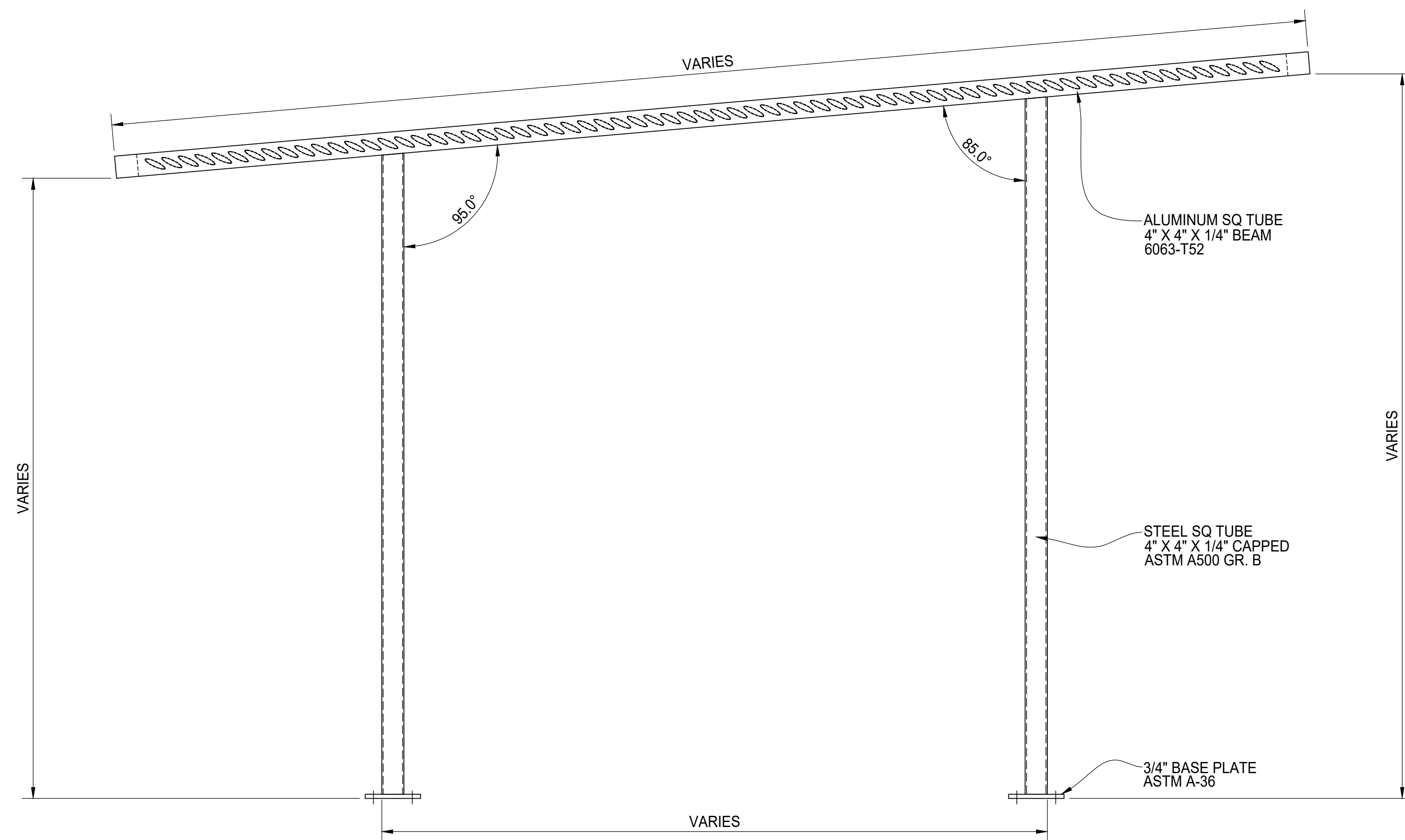
FRONT ELEVATION
