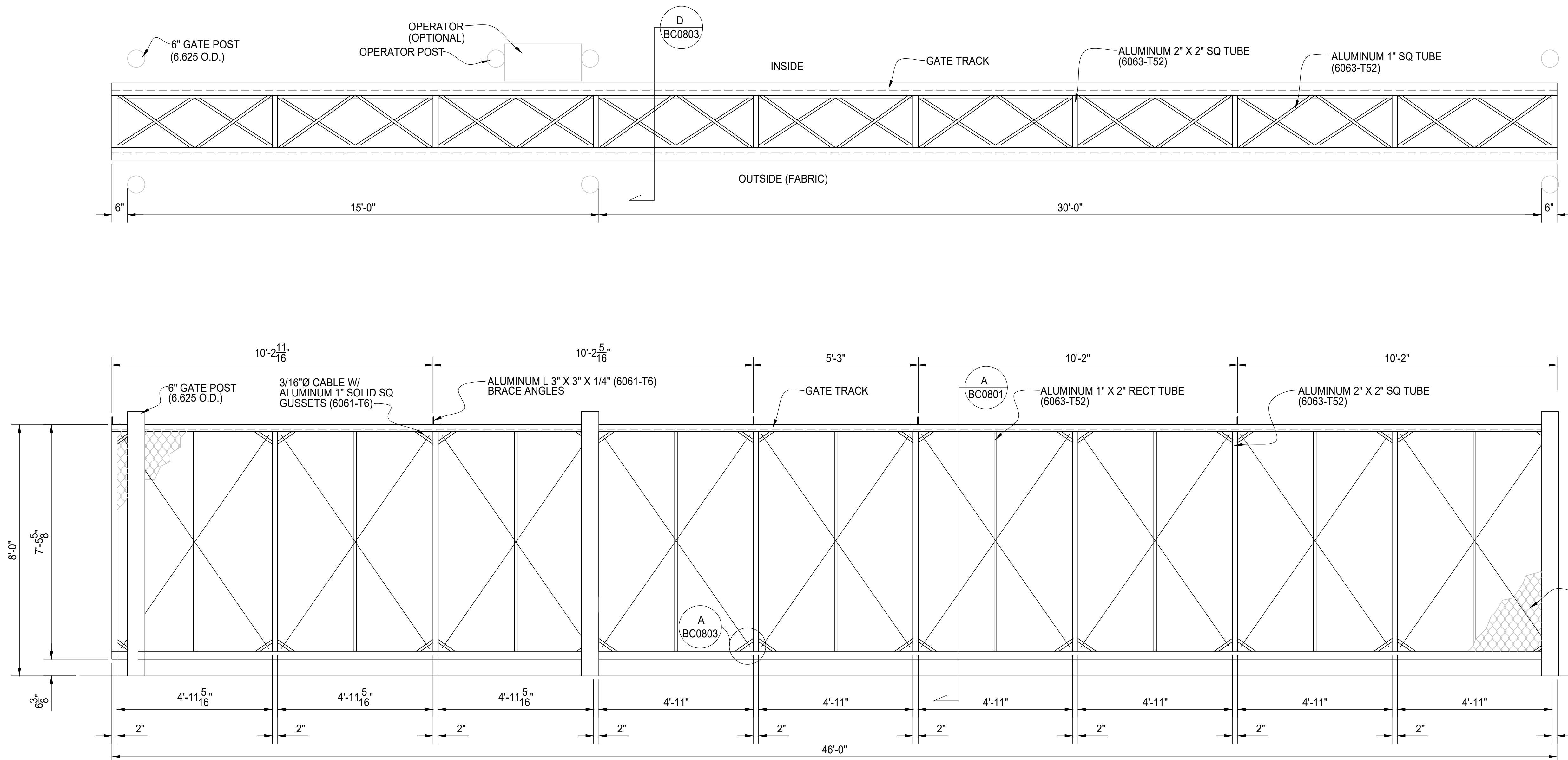
ELEVATION VIEW OF ALUMINUM BOX FRAME CANTILEVER OUTSIDE LOOKING IN, OPERATOR NOT SHOWN THIS VIEW
