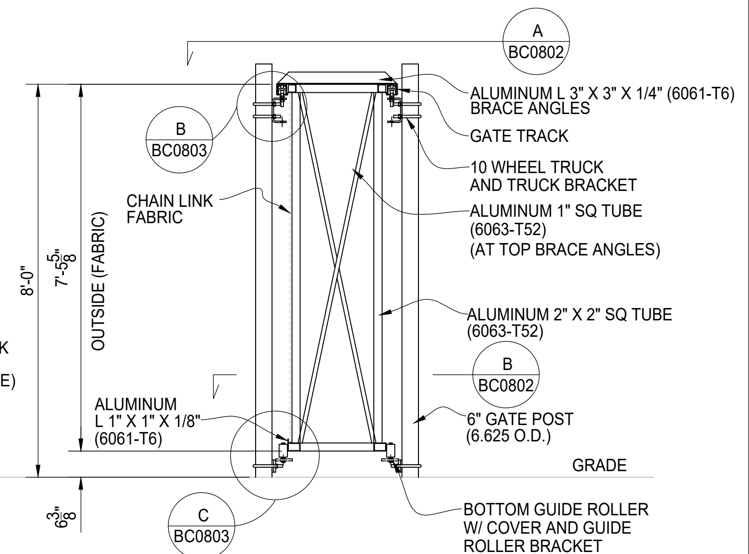
A SECTION VIEW OPERATOR NOT SHOWN THIS VIEW
