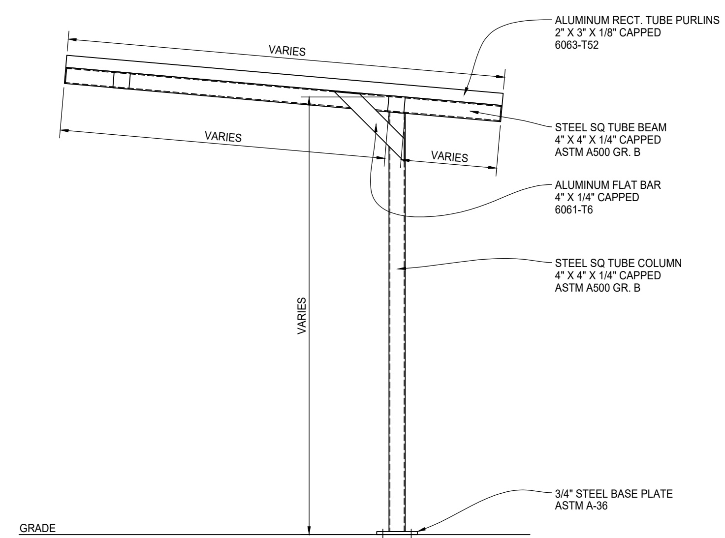
FRONT ELEVATION
