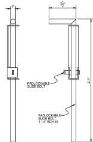
DROP ROD DETAIL
