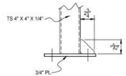
TYPICAL GUSSET DETAIL "ALUMINUM"
