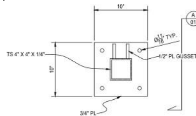
TYPICAL BASE PLATE DETAIL "ALUMINUM"
