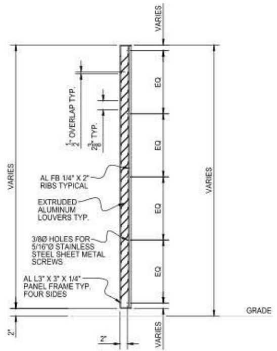
TYPICAL PANEL SECTION
