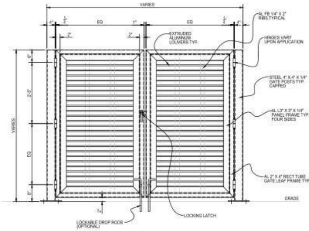
ELEVATION VIEW
