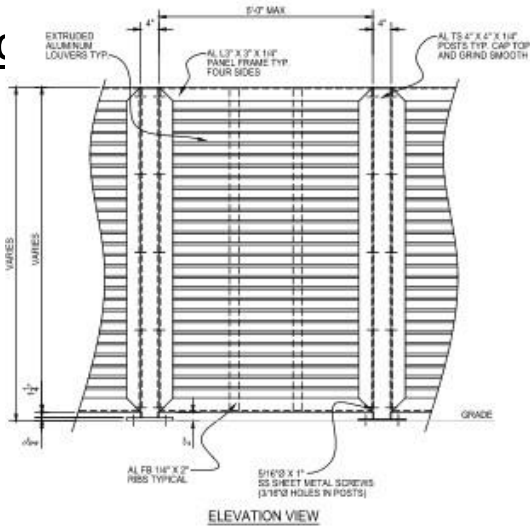
TYPICAL PANEL DETAIL
