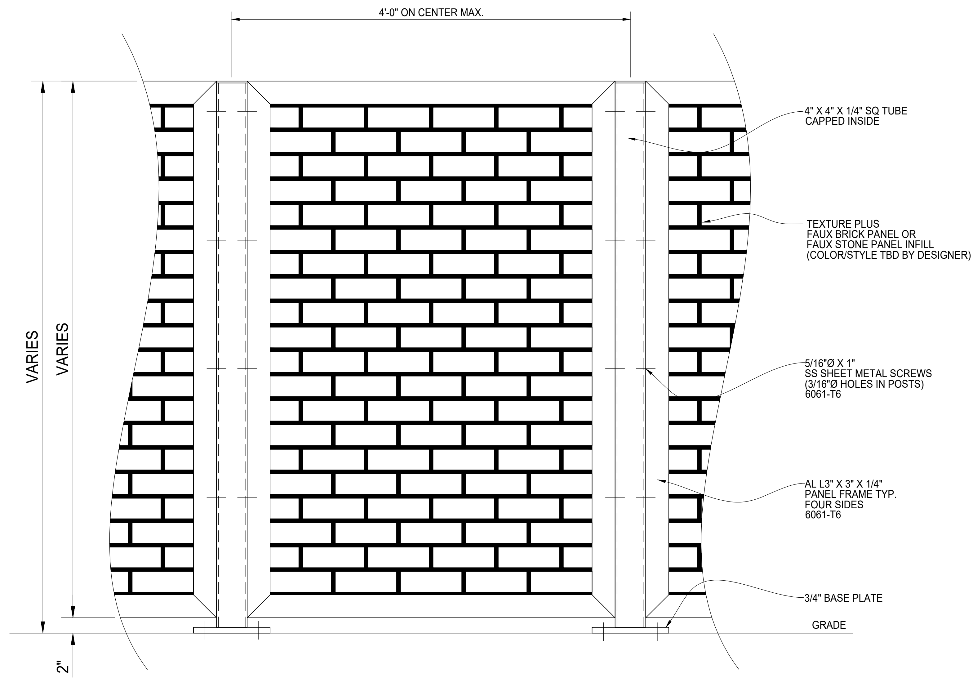
ELEVATION VIEW
