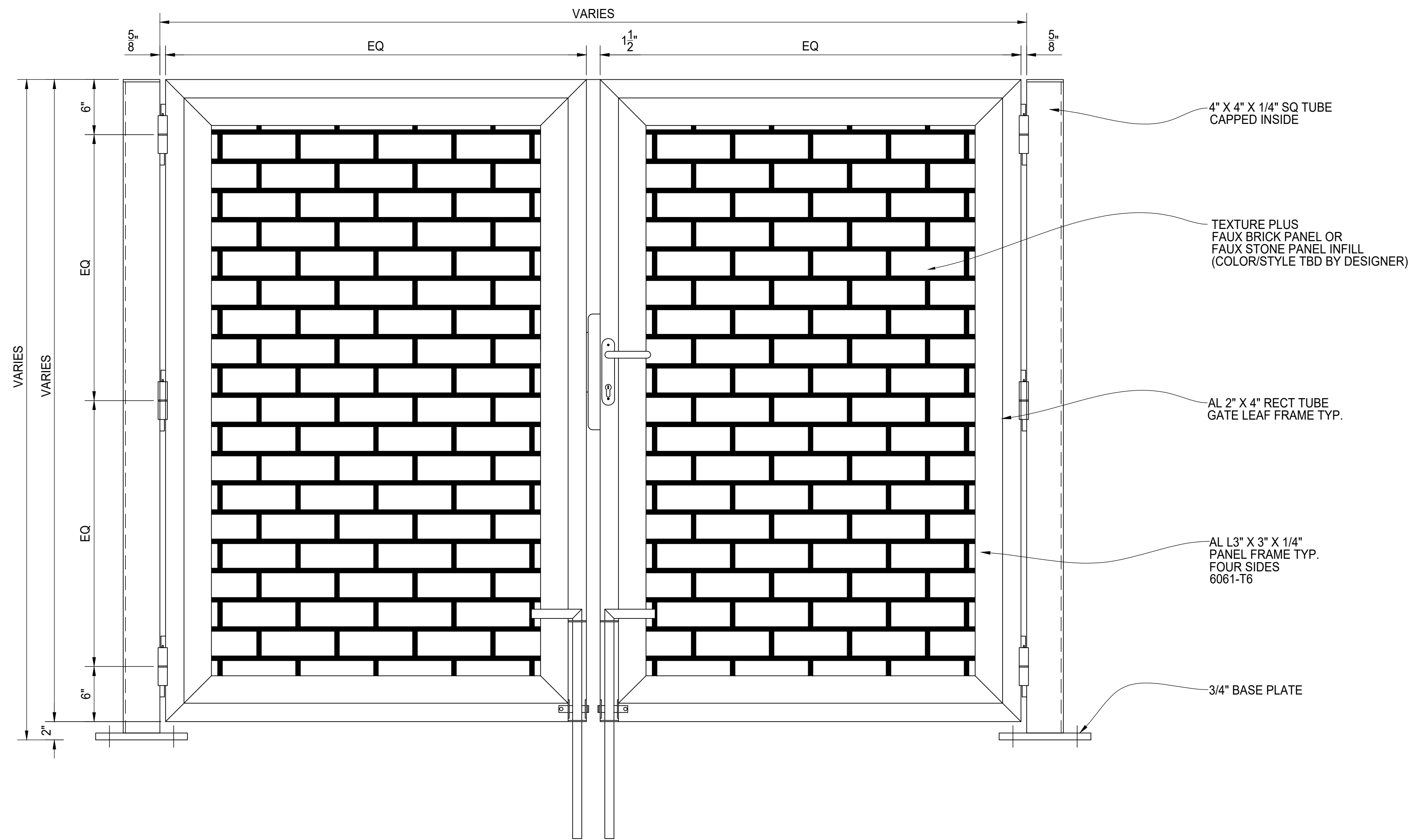
ELEVATION VIEW
