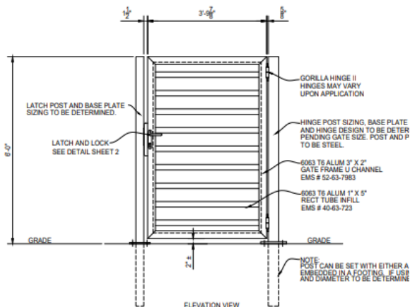
SINGLE SWING GATE ASSEMBLY HINGE SIDE AND OPENING DIRECTION MAY VARY SEE DETAIL SHEET 2 FOR HINGE AND LATCH
