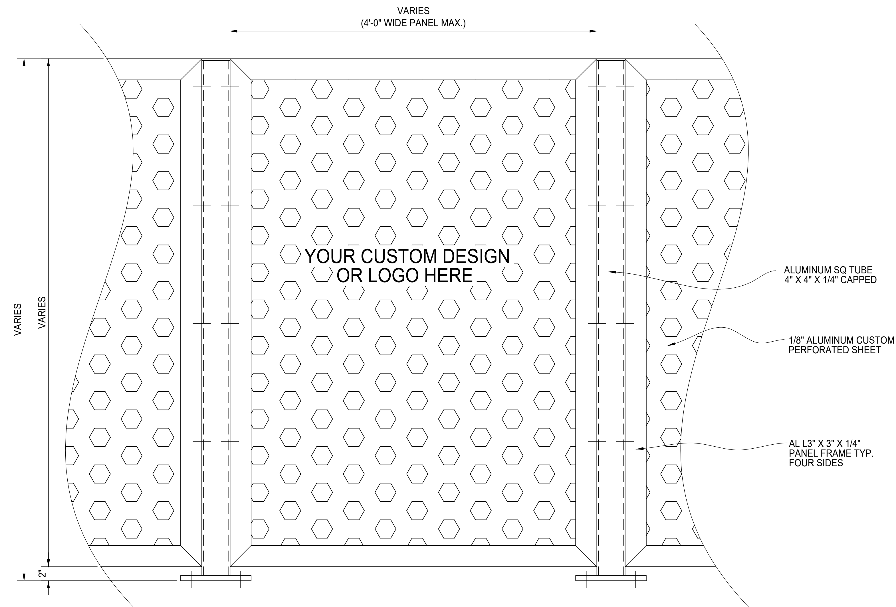
PANEL ELEVATION
