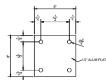
TYPICAL BASE PLATE DETAIL AT ALUMINUM POSTS ONLY. BASE PLATES AT STEEL HINGE POSTS TO BE NOTED PER LATH
