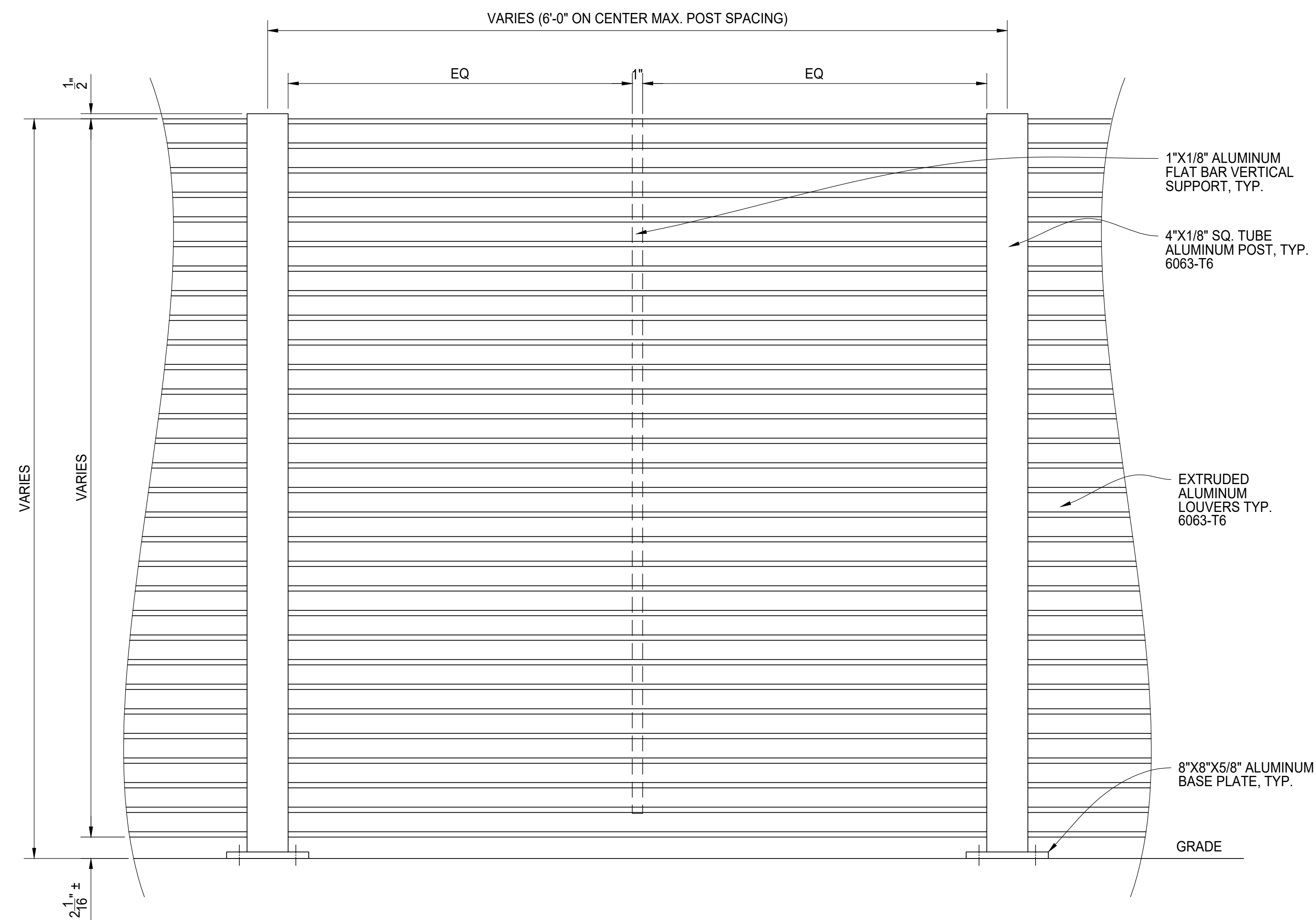
TYPICAL PANEL ELEVATION
