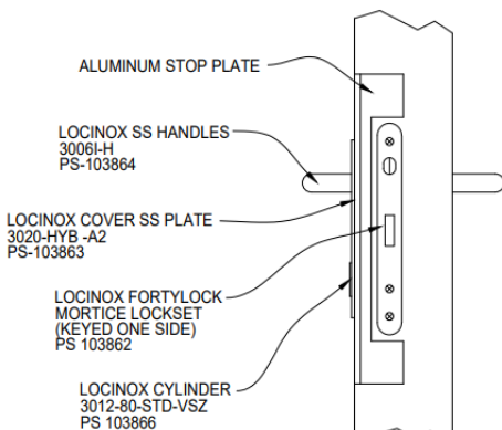
SIDE
