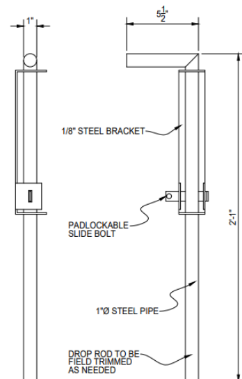
DROP ROD DETAIL
