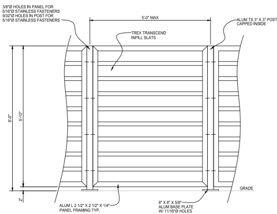
TYPICAL PANEL/POST DETAIL
