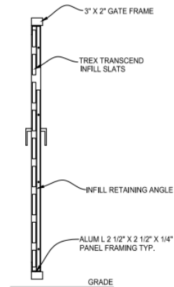
TYPICAL GATE SECTION
