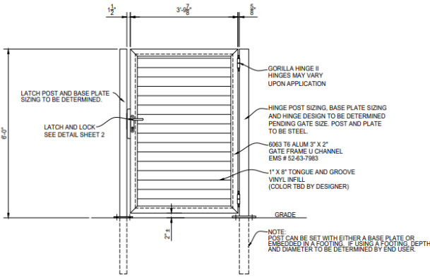
ELEVATION VIEW SINGLE SWING GATE ASSEMBLY HINGE SIDE AND OPENING DIRECTION MAY VARY SEE DETAIL SHEET 2 FOR HINGE AND LATCH
