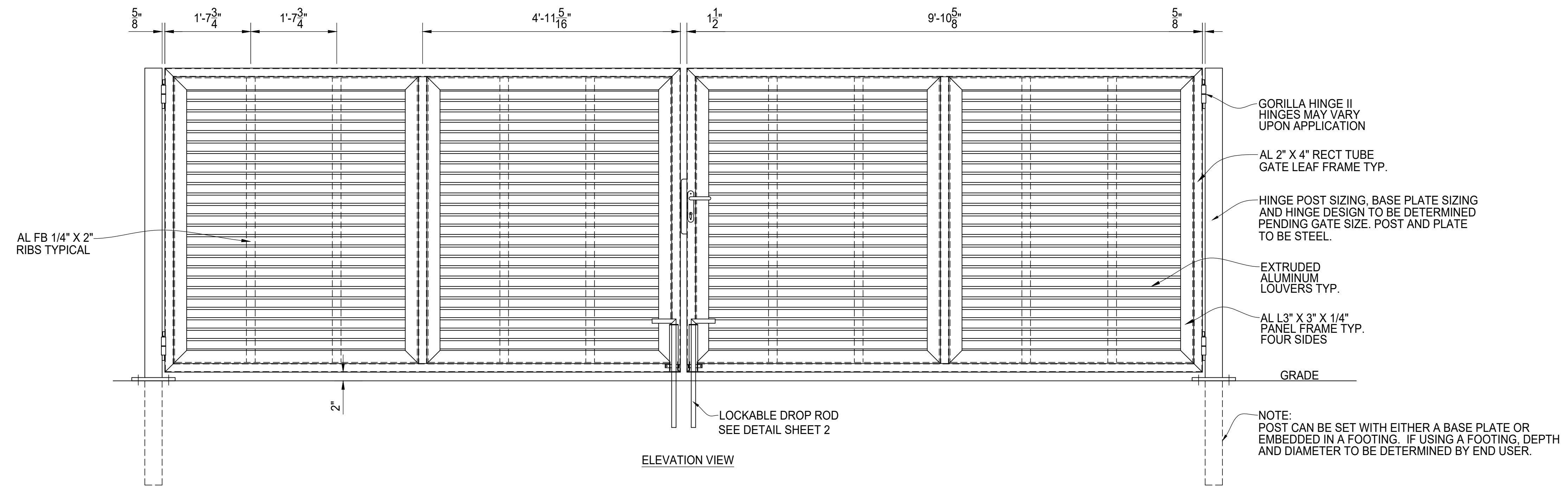
DOUBLE DRIVE GATE ASSEMBLY SEE DETAIL SHEET 2 FOR HINGE, LATCH AND DROP ROD
