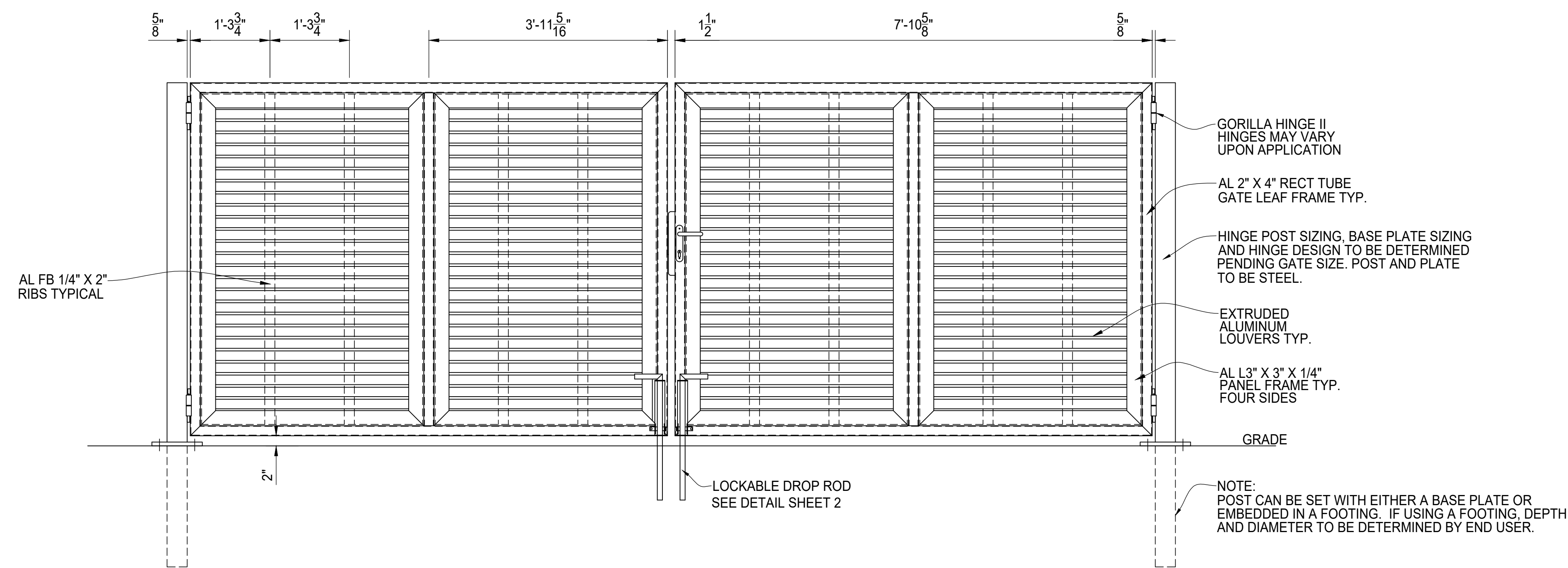
ELEVATION VIEW
