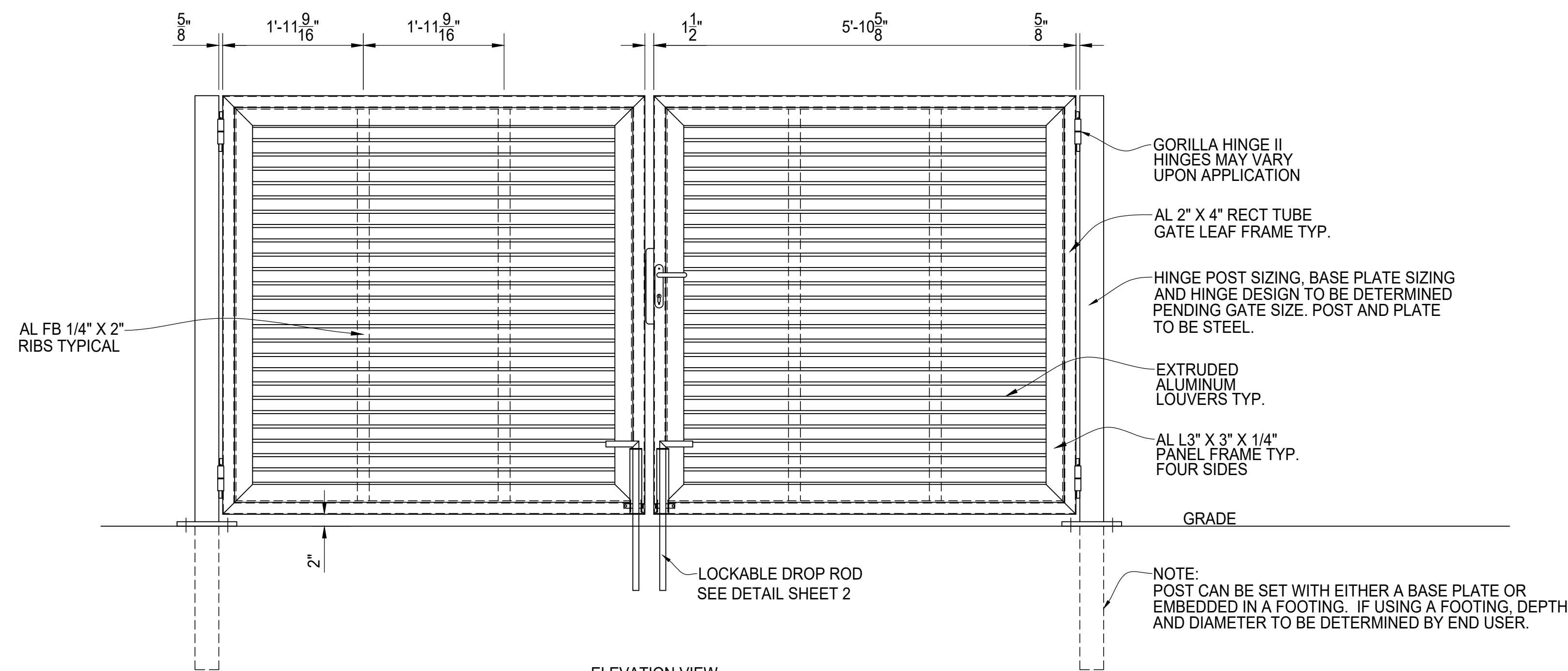
ELEVATION VIEW
