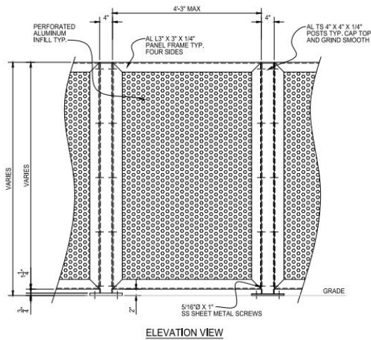
TYPICAL PERFORATED INFILL PANEL DETAIL 1/8" THICK ALUMINUM W/ 1"Ø HOLES ON 1 1/4" CENTERS (58% OPEN)
