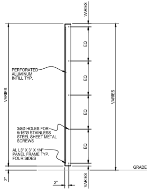
TYPICAL PANEL SECTION
