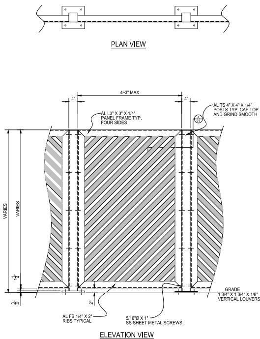
TYPICAL WIRE MESH INFILL PANEL DETAIL ALUM 1 3/4" X 1 3/4" X 1/8" ANGLE VERTICAL LOUVERS
