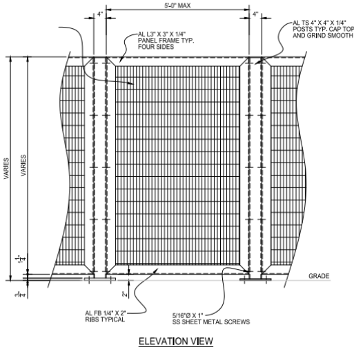
TYPICAL BAR GRATING INFILL PANEL DETAIL 1/8" THICK X 1" ALUMINUM BARS ON 1 3/16" CENTERS
