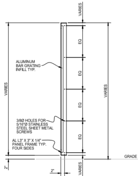
1/8" THICK X 1" ALUMINUM BARS ON 1 3/16" CENTERS
