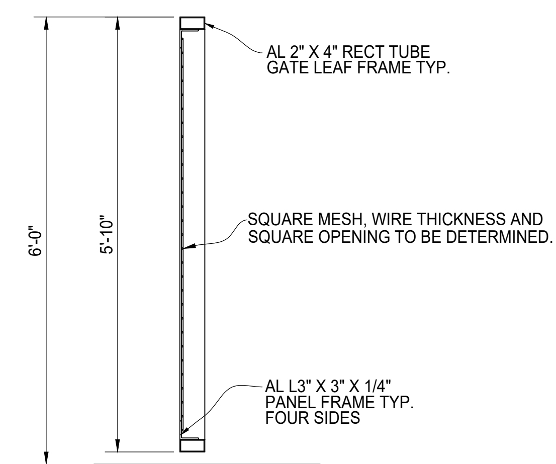
SIDE VIEW GATE SECTION
