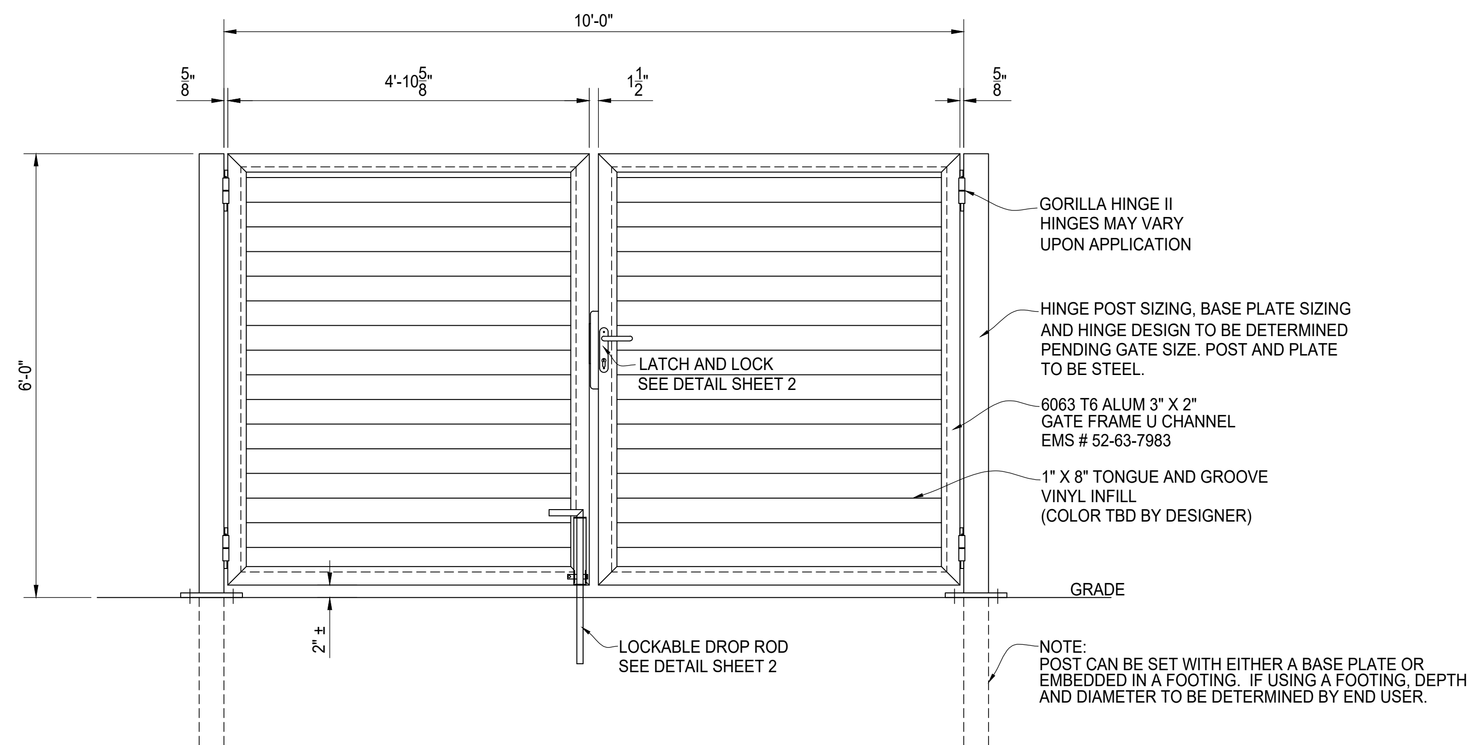
ELEVATION VIEW
