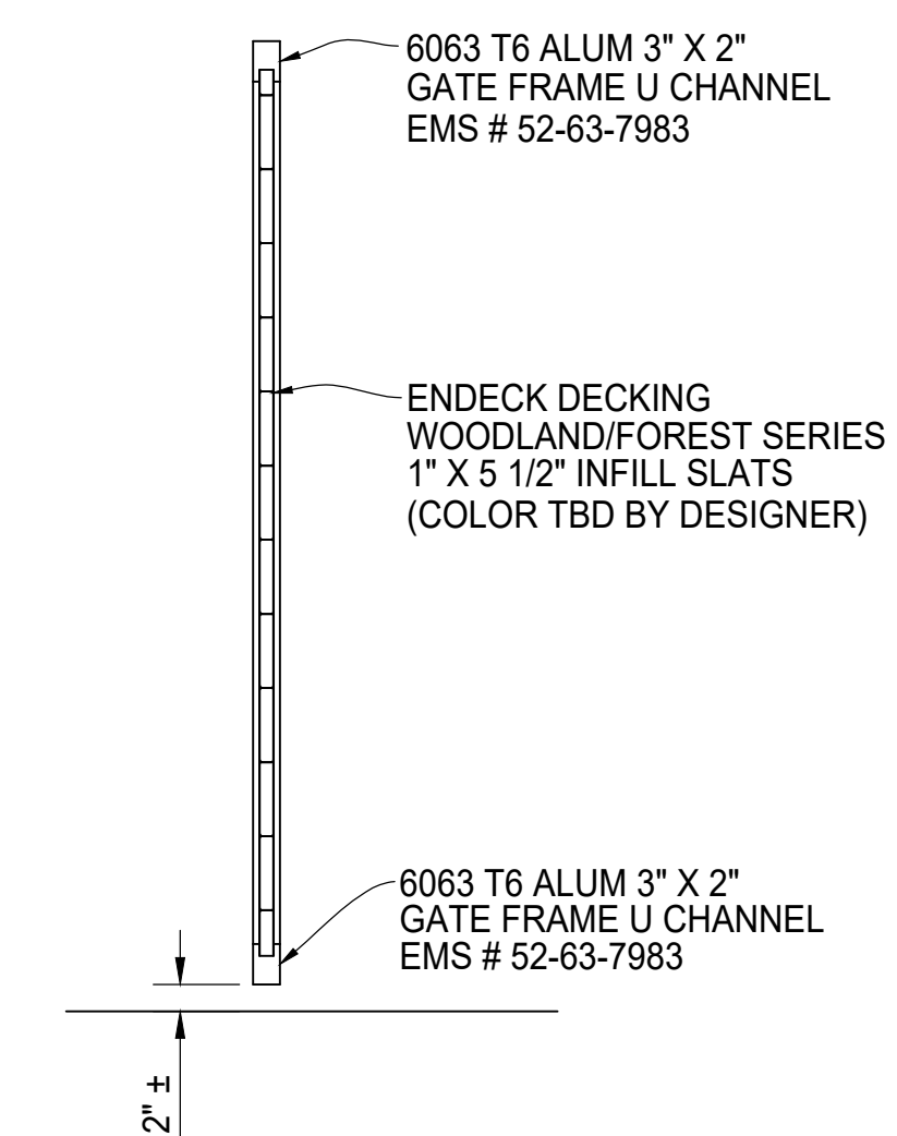
SIDE VIEW
