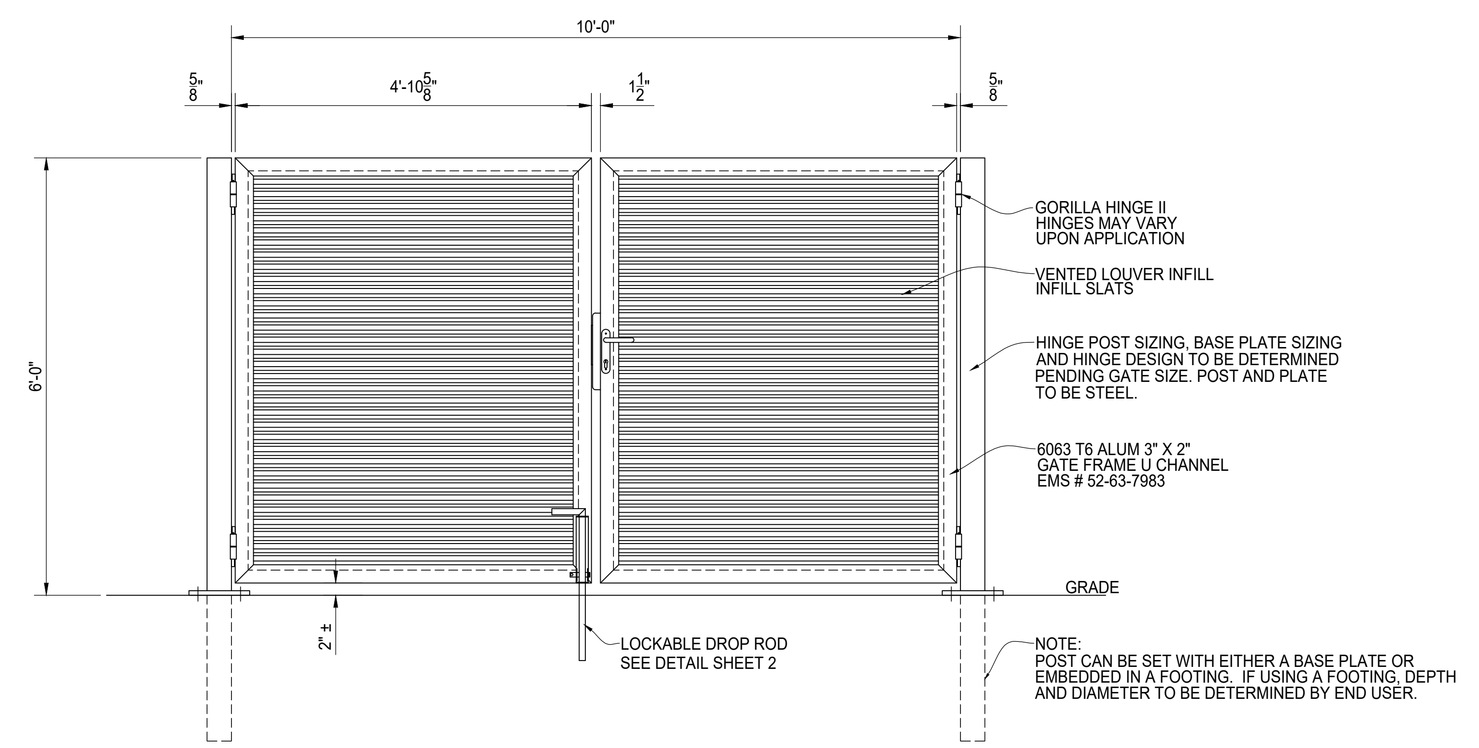
ELEVATION VIEW
