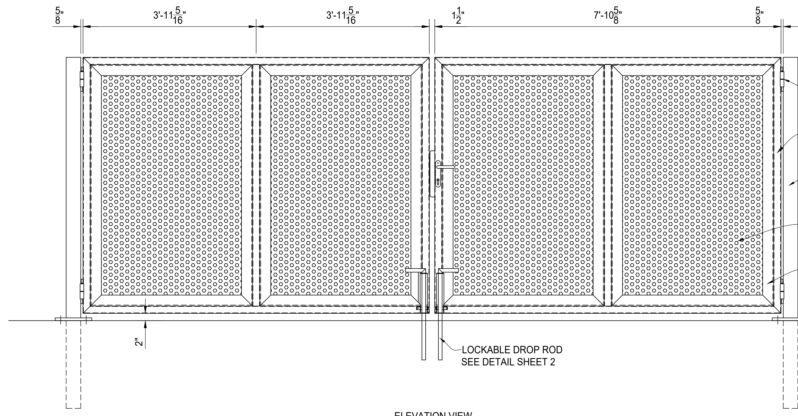
ELEVATION VIEW
