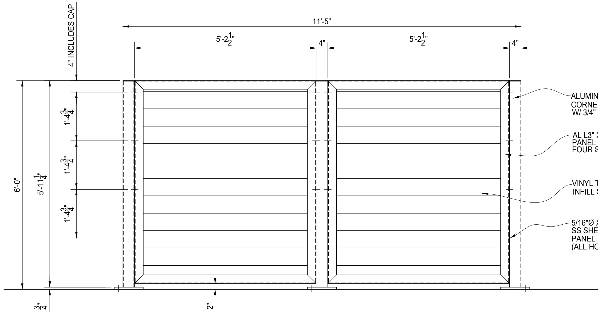
A REAR ELEVATION VIEW
