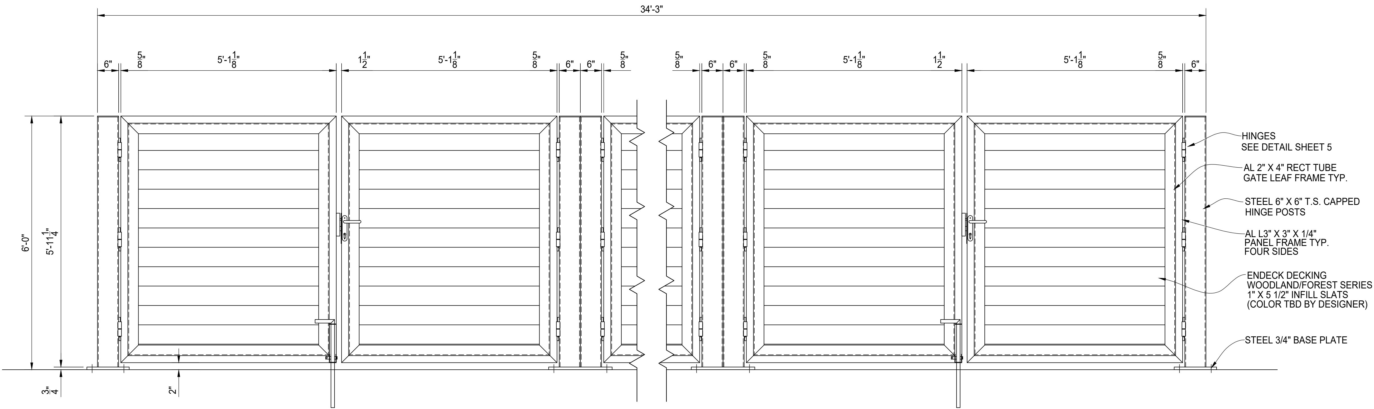
A GATE ELEVATION VIEW SEE SHEET 05 FOR HINGE, LATCH AND DROP ROD DETAILS
