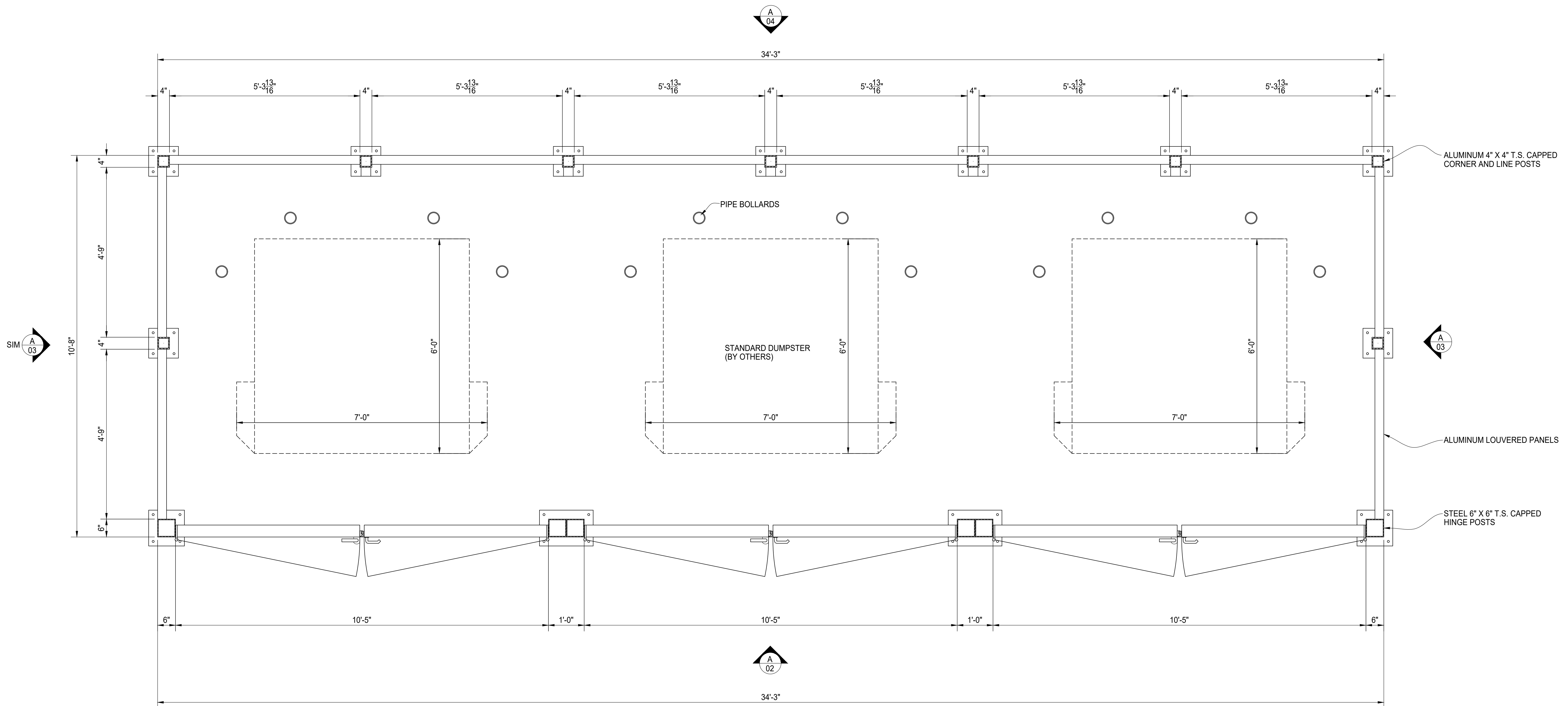
PLAN VIEW @ DUMPSTER ENCLOSURE
