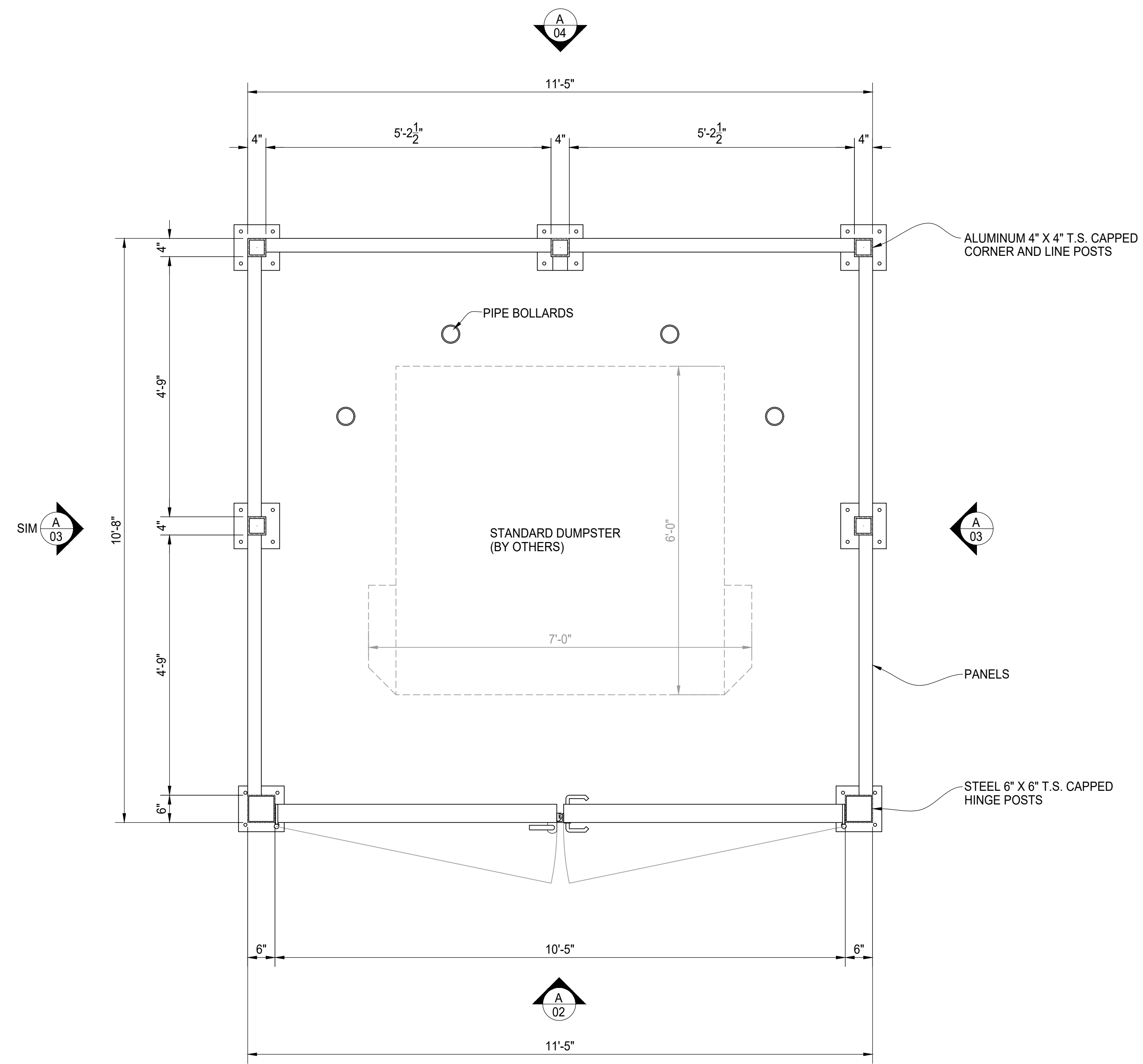
PLAN VIEW @ DUMPSTER ENCLOSURE
