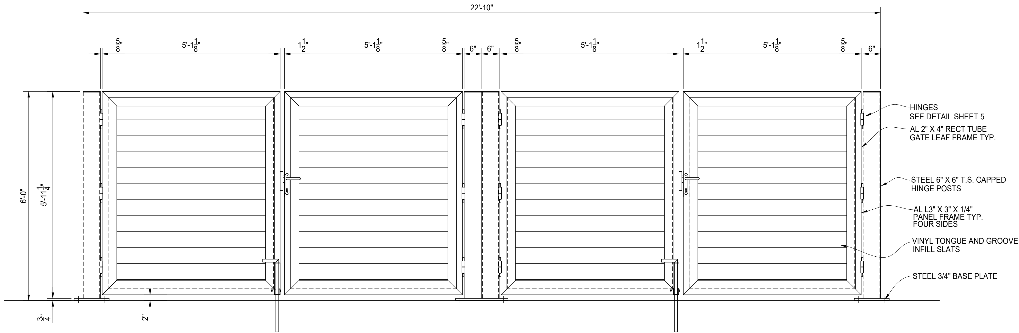
A GATE ELEVATION VIEW SEE SHEET 05 FOR HINGE, LATCH AND DROP ROD DETAILS
