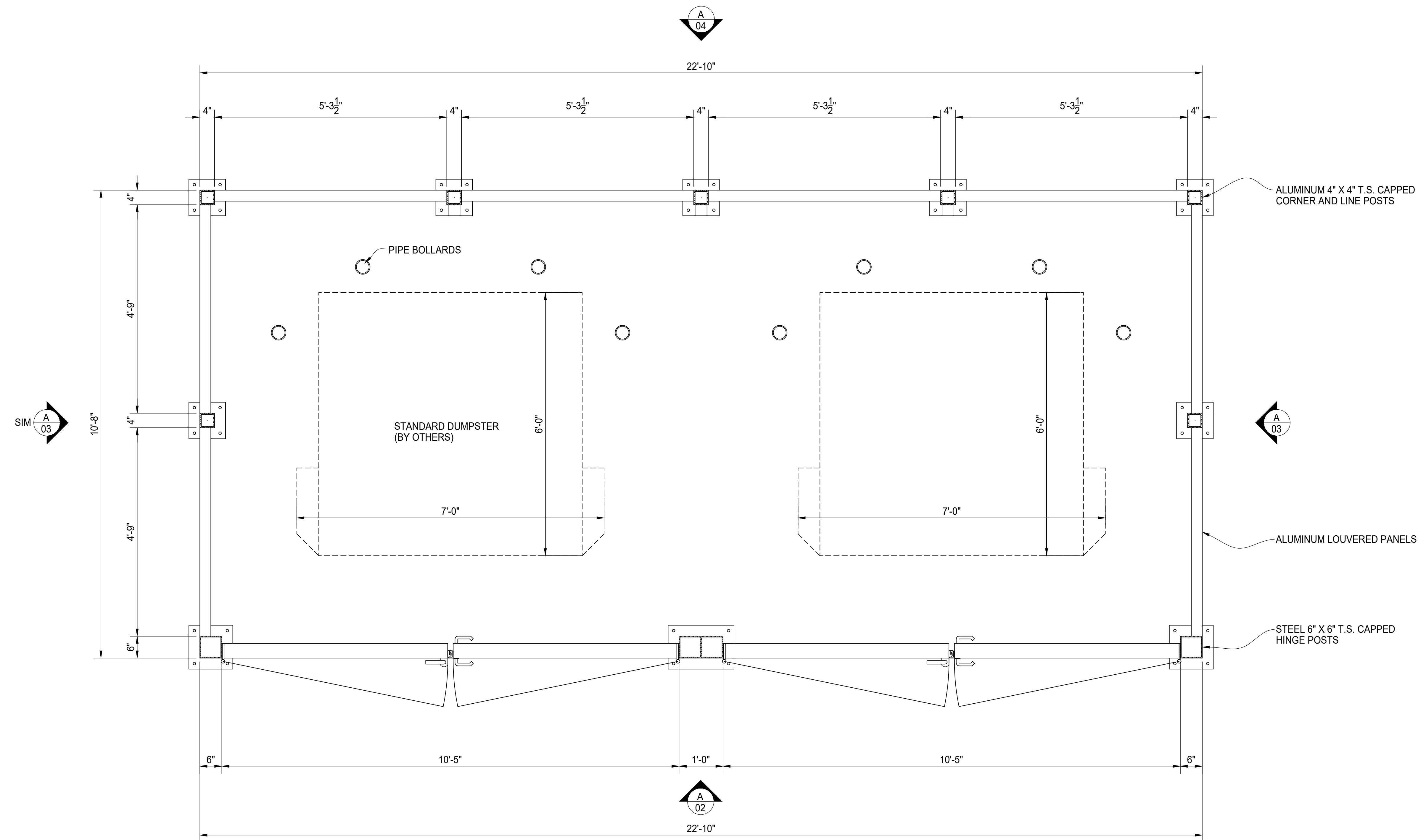
PLAN VIEW @ DUMPSTER ENCLOSURE
