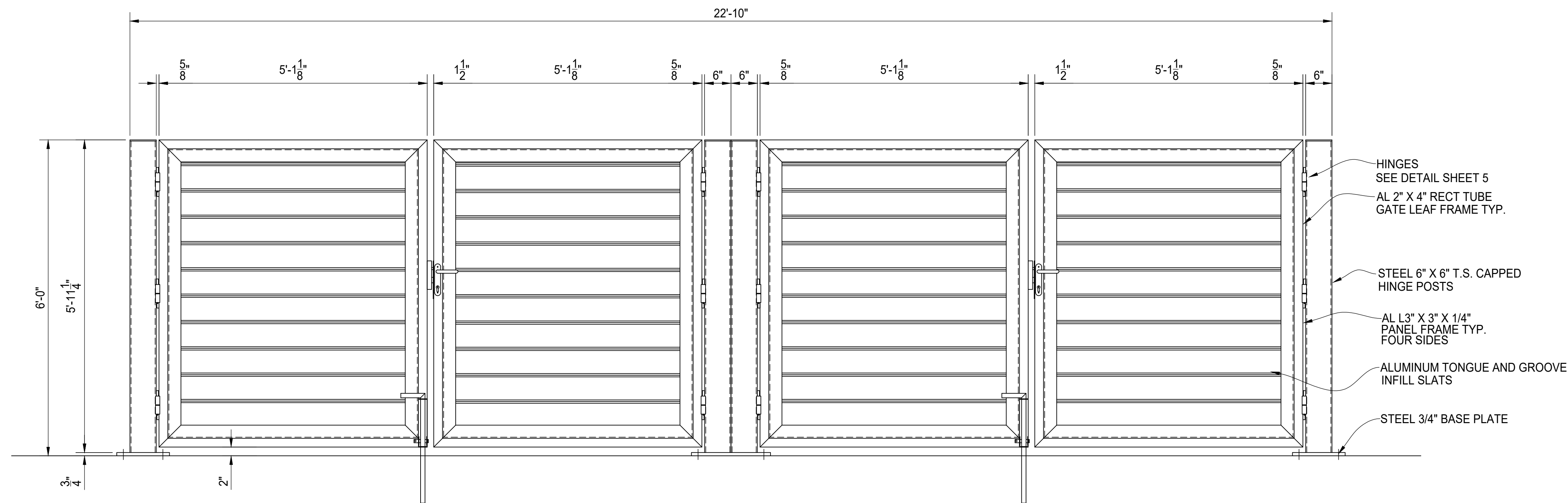
A GATE ELEVATION VIEW SEE SHEET 05 FOR HINGE, LATCH AND DROP ROD DETAILS
