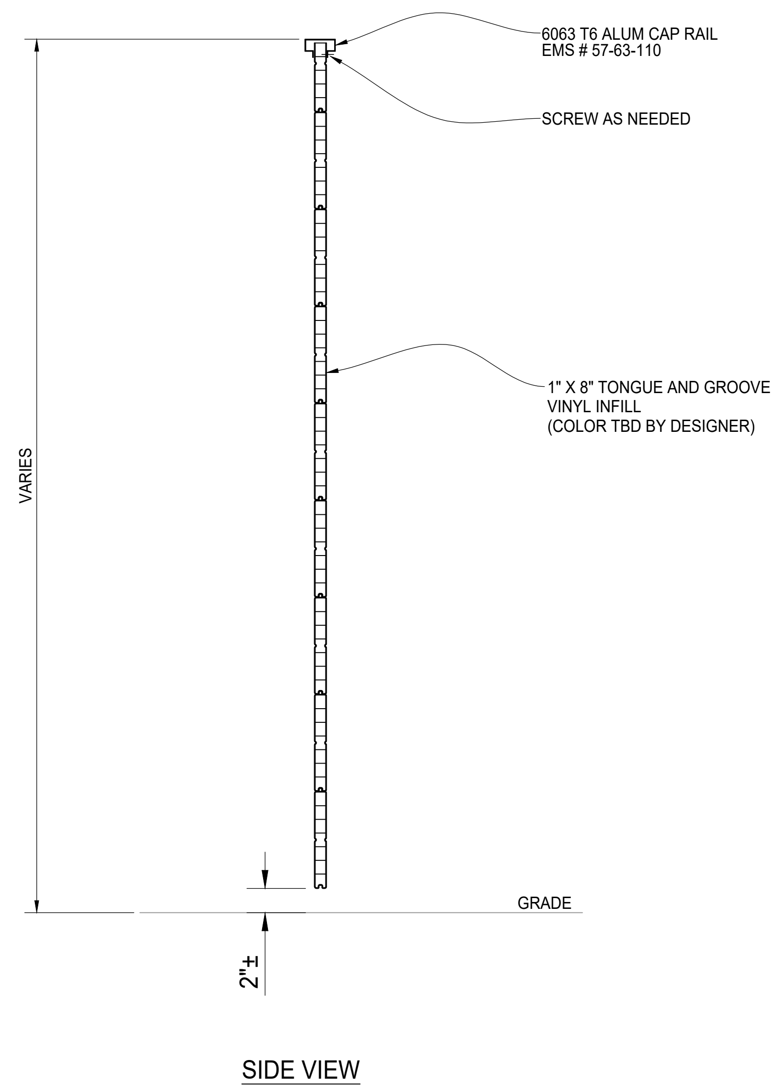
PANEL SECTION
