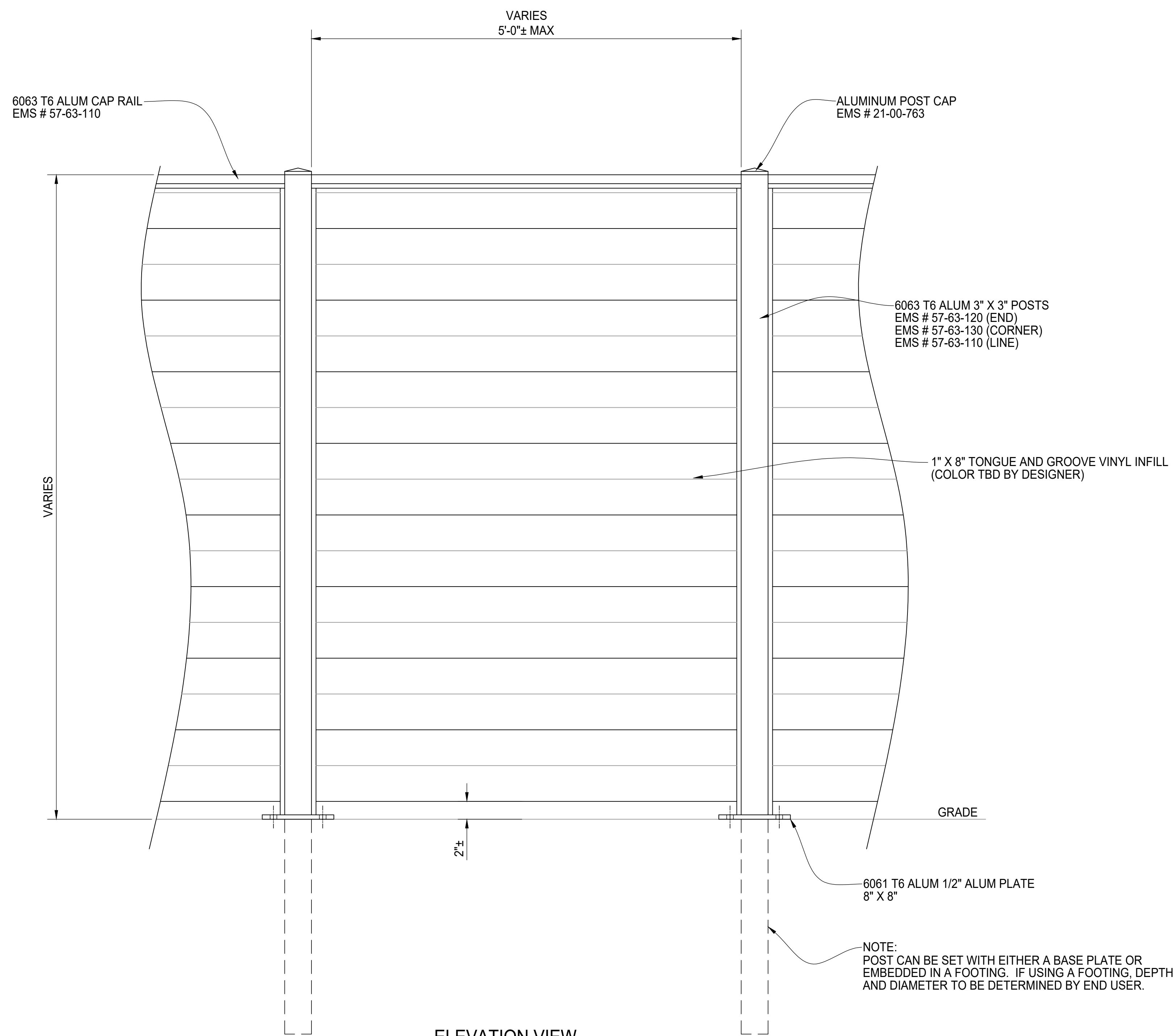
ELEVATION VIEW
