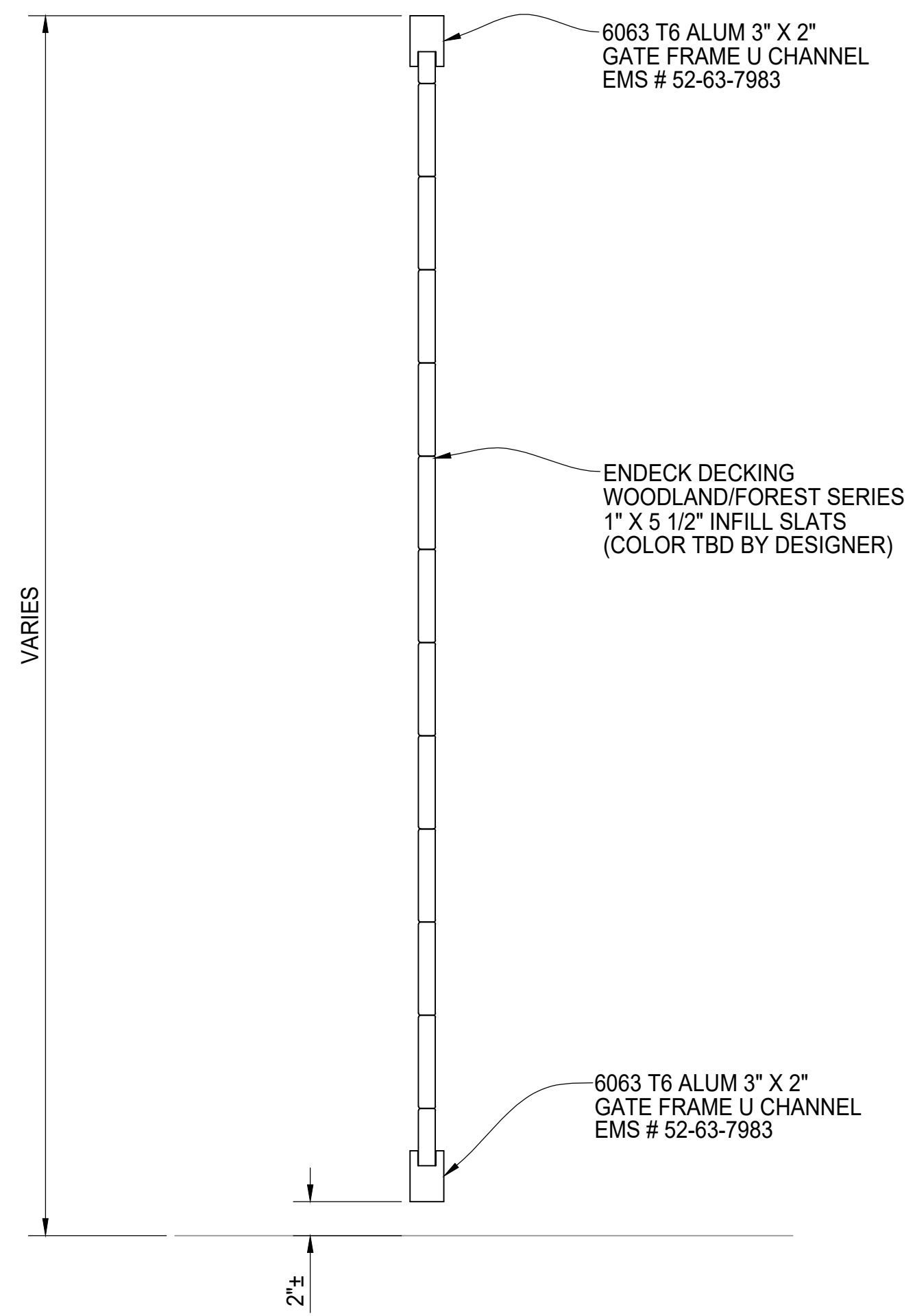
SIDE VIEW
