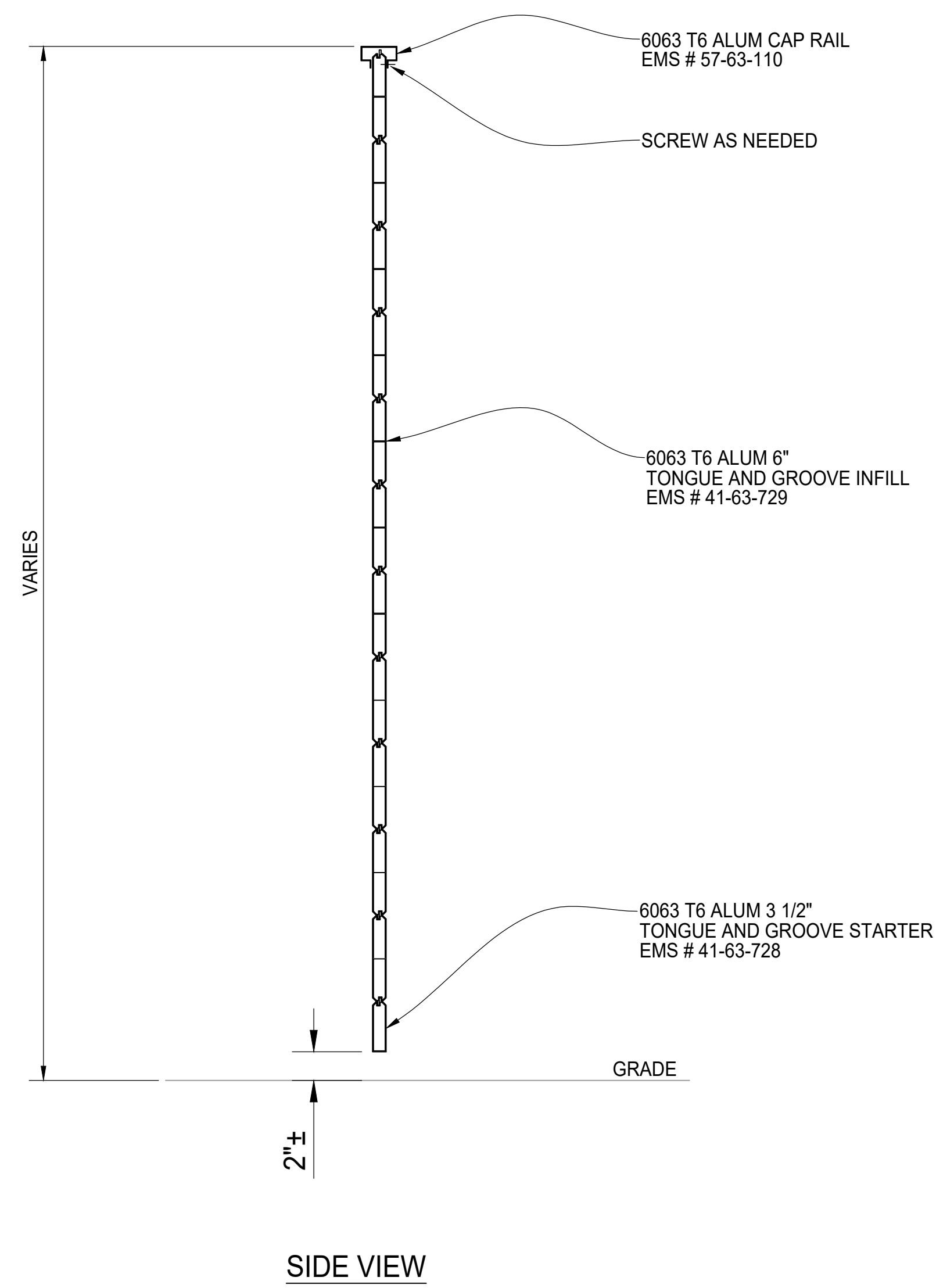
PANEL SECTION
