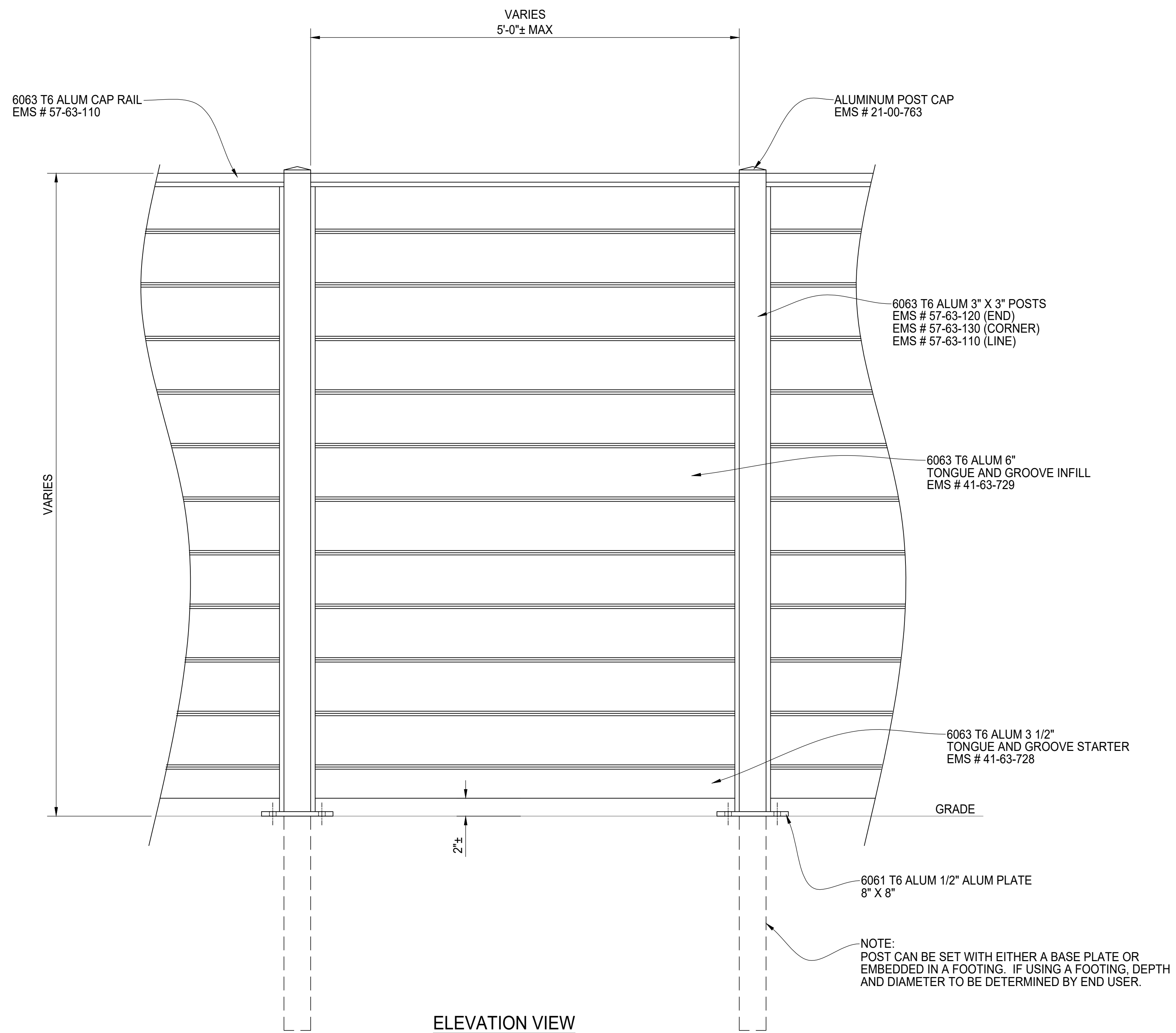
TYPICAL PANEL AND POST DETAIL
