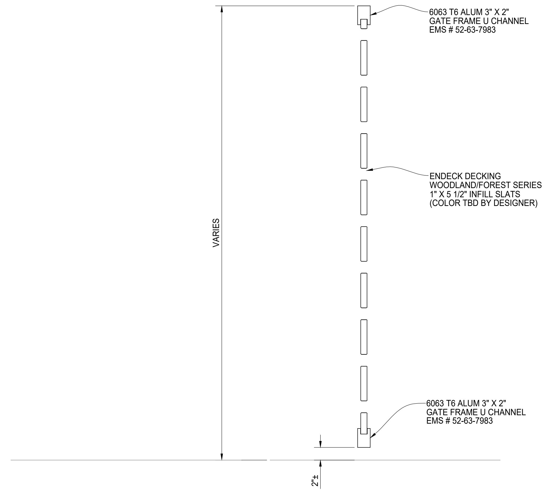
SIDE VIEW
